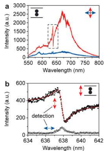
FIGURE 5. (a) Fluorescence spectrum from the configuration shown in Figure 4a (see inset) with the excitation light polarized perpendicular (red) or parallel (blue) to the waveguide axis, respectively. No polarization filtering is applied in the detection path. (b) Resonance peak of mode M1 for the same configuration as in (a). The system is excited along the nanosphere alignment direction and additional polarization filtering perpendicular (filled circles) or parallel (open circles) to the waveguide axis is applied in the detection path. A Fano-type function (red curve, eq 3) is used to fit the data, which was flattened through normalization to the unstructured background prior to fitting.
