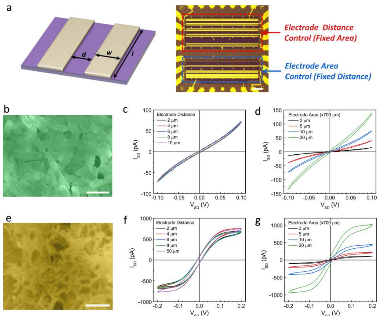
Figure 3. Nanoelectronic investigation of the “electrical conduction” of Shewanella and Geobacter biofilms using electrode pairs with varying gaps and areas. (a) Schematic illustration of the biofilm measurements using two sets of pair electrodes with either varying gaps (with fixed areas) or varying electrode areas (with fixed gaps). (b) Representative SEM image of a Shewanella biofilm. (c, d) I_{SD} – V_{SD} behavior of living Shewanella biofilms with different pair electrode distances (c) and different electrode areas (d). (e) Representative SEM image of a Geobacter biofilm grown under anaerobic conditions. (f, g) I_{SD} – V_{SD} behavior of living Geobacter biofilms with different electrode distances (f) and different electrode areas (g). Scale bars in (b) and (e) are 2 \mu\text{m} .
