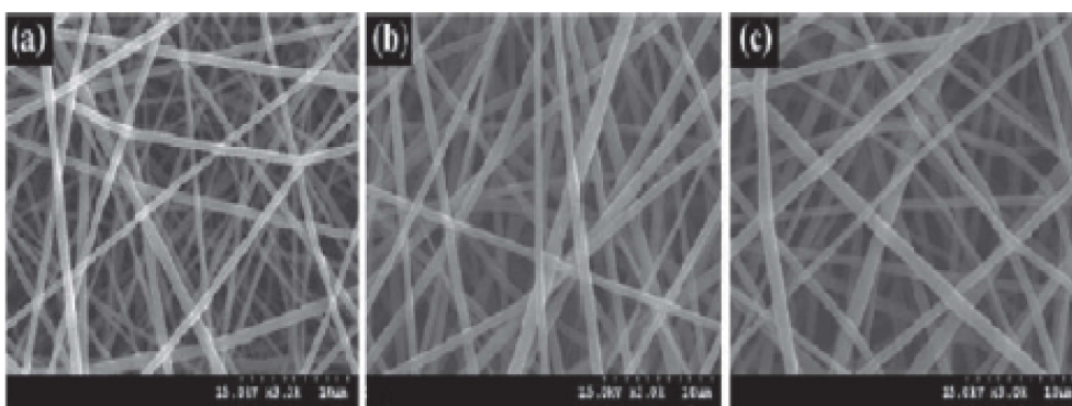
Figure 2. SEM micrographs of electrospun nanofibrous scaffolds using a PHBV/gelatin solution at TFE 6 wt%; (a) 30/70, (b) 50/50, and (c) 70/30 (adapted from reference 127).
