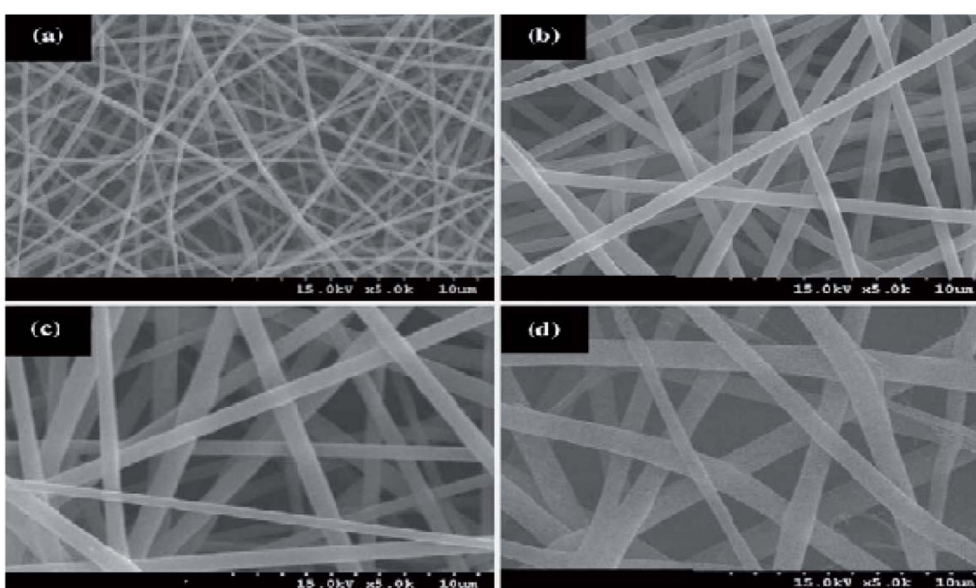
Figure 3. SEM micrographs of electrospun nanofibrous scaffolds using TFE solutions with different amount of PHBV/gelatin (50/50); (a) 2 wt%, (b) 4 wt%, (c) 6 wt%, and (d) 8 wt% (adapted from reference 127).
