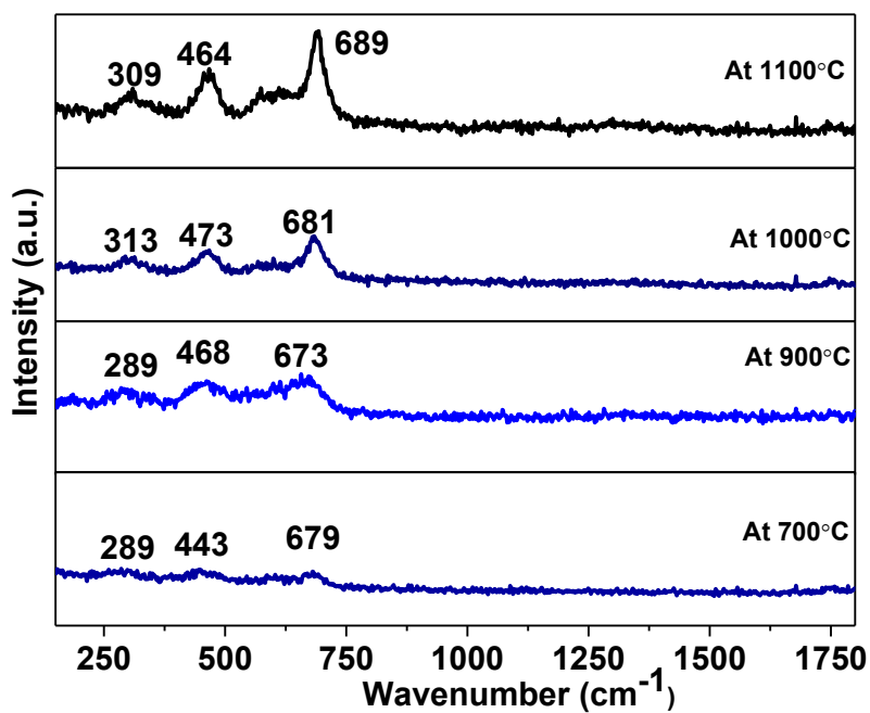
Figure 3. Raman Active Modes of CoFe 2 O 4 nanoparticles as a function of temperature (1100 0 C – 700 0 C).
