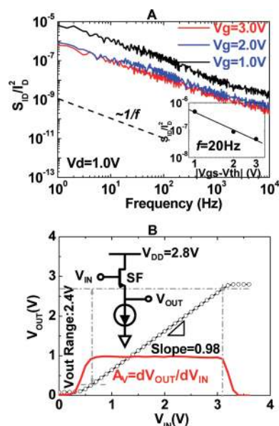
FIGURE 4. Low-frequency noise behavior and SF performance of a -IGZO TFT with W/L=180 nm/250 nm. (A) Normalized drain-current noise power spectral density ( S_{ID}/I_D^2 ) versus frequency with V_{GS} increasing from 1.0 to 3.0 V and for a constant V_{DS} of 1.0 V. The inset shows the normalized S_{ID}/I_D^2 versus the gate voltage overdrive |V_{GS}-V_{th}| at a frequency of 20 Hz. (B) V_{OUT} versus V_{IN} of a SF-based a -IGZO TFT with W/L=180 nm/250 nm. The red line indicates the derivative of V_{OUT} with respect to V_{IN} . The inset shows the circuit schematics of the SF at a V_{DD} of 2.8 V.
