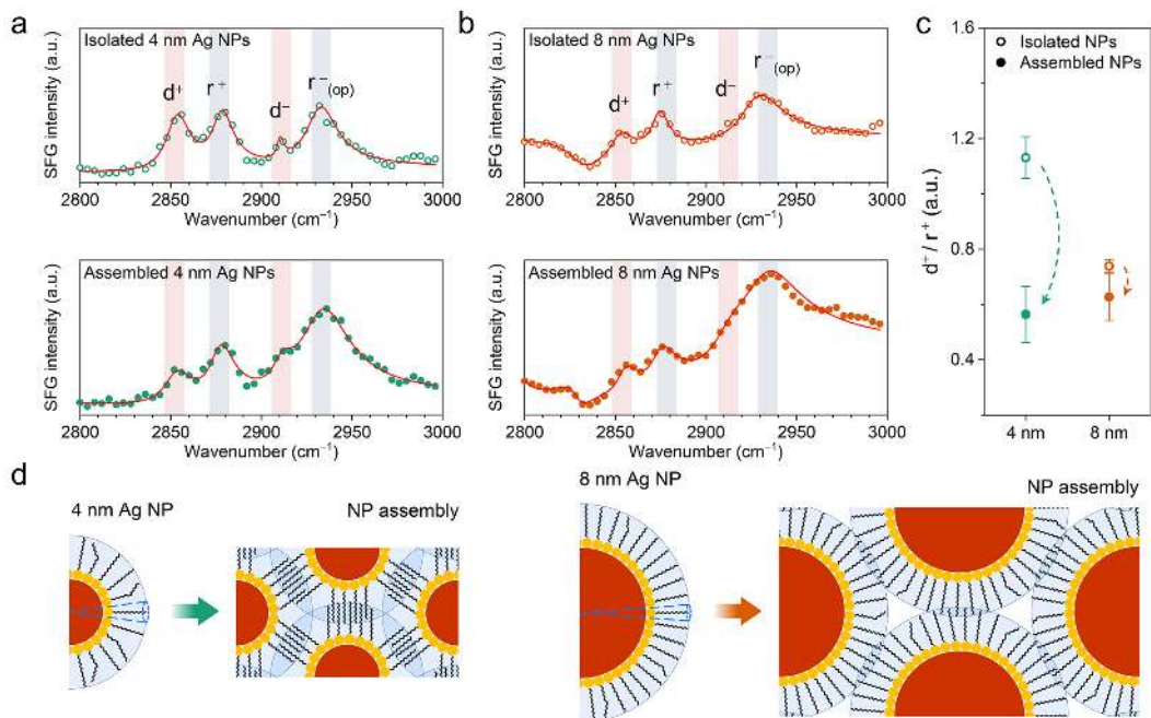
Figure 4. Nanoparticle assembly induced ligand interdigitation. a , b , Sum frequency generation (SFG) spectra of isolated (top) and assembled (bottom) 4 nm ( a ) and 8 nm ( b ) Ag NPs. Red curves are fitted lines (see Methods for details about fitting). c , SFG peak amplitude ratio of methylene symmetric stretch ( d^+ ) to methyl symmetric stretch ( r^+ ) before and after assembly of 4 and 8 nm Ag NPs. d , Schematics illustrating the impact of nanoparticle surface curvature on ligand interdigitation. Blue dashed lines indicate cylindrical space available for individual ligands before NP assembly.
