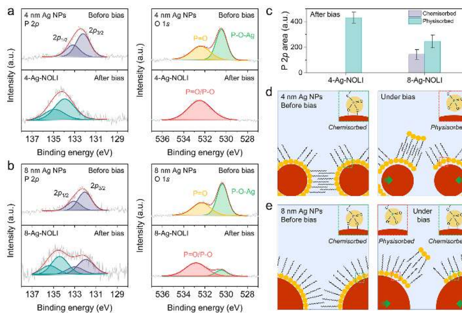
Figure 5. Formation of a ligand layer under bias from interdigitated ligands. a, b, X-ray photoelectron spectroscopy (XPS) P 2 p and O 1 s spectra of the assembled 4 nm ( a ) and 8 nm ( b ) Ag NPs, and the resultant 4-Ag-NOLI ( a ) and 8-Ag-NOLI ( b ) after 2 min of bias at -0.68 V vs. RHE. P 2 p peaks were deconvoluted into 2p_{1/2} and 2p_{3/2} . Purple in the P 2 p XPS spectra represents the chemisorbed state of ligands, while cyan represents the physisorbed state. Likewise, green (P-O-Ag) in the O 1 s XPS spectra indicate the chemisorbed ligand state, while pink (P=O/P-O) represents the physisorbed state. c, P 2 p peak area integrated after bias for 2 min. The peaks representing chemisorbed and physisorbed ligand states were separately integrated. d, e, Schematics illustrating the behavior of interdigitated ligands under bias for the assembled 4 nm ( d ) and 8 nm ( e ) Ag NPs. Insets show the binding states of ligands before and under bias for each case. Green arrows indicate the motion of Ag NPs under bias resulting in NP fusion. Only two particles are shown for clarity in each case.
