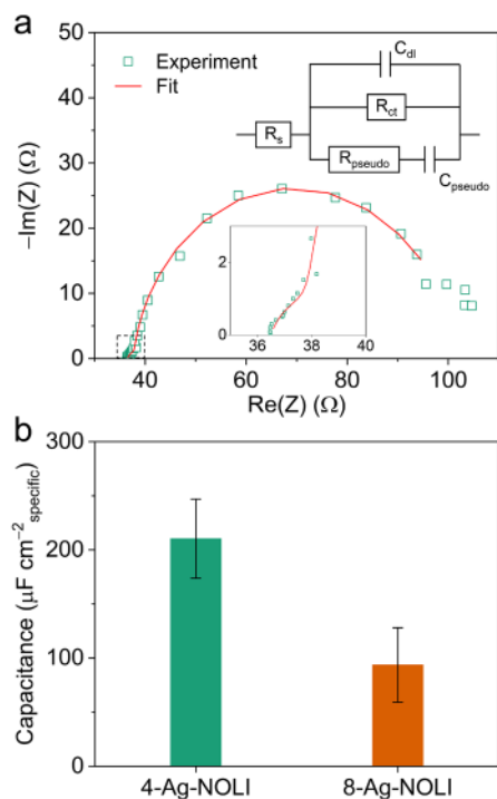
Figure 7. Pseudocapacitive characteristics and specific capacitance comparison of the NOLI for Ag-NOLI catalysts. a , Representative Nyquist plot of 4-Ag-NOLI obtained at -0.68 V vs. RHE. Insets show the equivalent circuit diagram used to fit the impedance data (top), and a high frequency region of the Nyquist plot (bottom). The equivalent circuit is composed of solution resistance ( R_s ), double layer capacitance ( C_{dl} ), charge transfer resistance ( R_{ct} ), pseudocapacitance ( C_{pseudo} ), and charger transfer resistance for pseudocapacitance ( R_{pseudo} ). b , Specific capacitance measured for the Ag-NOLI catalysts.
