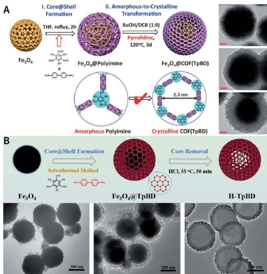
Fig. 38 (A) Preparation protocol and HRTEM images of \text{Fe}_3\text{O}_4@\text{COF}(\text{TpBD}) with shell thicknesses of 20, 50, and 100 nm. Scale bar: 50 nm. Adapted with permission. 232 Copyright 2016, Wiley-VCH Verlag GmbH & Co. KGaA, Weinheim. (B) Synthesis protocol and HRTEM images of hollow COF nanoshells. Adapted with permission. 233 Copyright 2018, Elsevier B.V.
