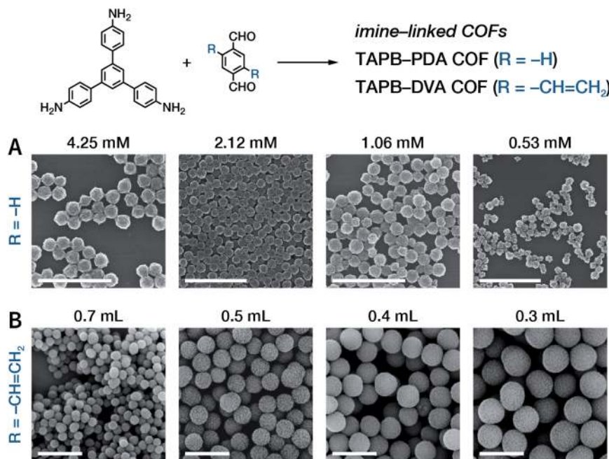
Fig. 36 SEM images of imine-linked COFs prepared in \text{CH}_2\text{CN} at room temperature. (A) TAPB-PDA COF with particle sizes of 200, 260, 290, and 330 nm prepared at varying aryltriamine monomer concentrations. Scale bar: 2 \mu\text{m} . Adapted with permission. 219 Copyright 2019, The Royal Society of Chemistry. (B) TAPB-DVA COF with particle sizes of 450, 800, 1000, and 1300 nm synthesized at different volumes of acetic acid. Scale bar: 2 \mu\text{m} . Adapted with permission. 222 Copyright 2019, American Chemical Society.
