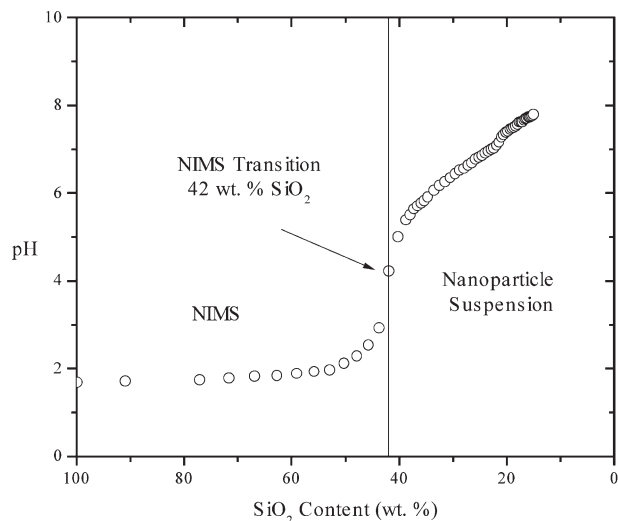
Figure 2. Titration curve for the reaction between surface modified silica and tertiary amine. The equivalence point for this system occurs at pH \sim 4 and corresponds to a SiO_2 concentration of 42 wt %.
