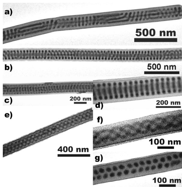
Figure 1. TEM images of native PS- b -P2VP nanorods released from AAO with pore diameters ranging from \approx 170 down to \approx 100 nm. The P2VP domains were selectively stained with I_2 and appear darker than the PS matrix. a) D \approx 170 nm, D/L_0 \approx 4.0 ; b)–d) D \approx 150 nm, D/L_0 \approx 3.5 ; e) D \approx 133 nm, D/L_0 \approx 3.1 ; f) D \approx 119 nm, D/L_0 \approx 2.8 ; g) D \approx 104 nm, D/L_0 \approx 2.4 .
