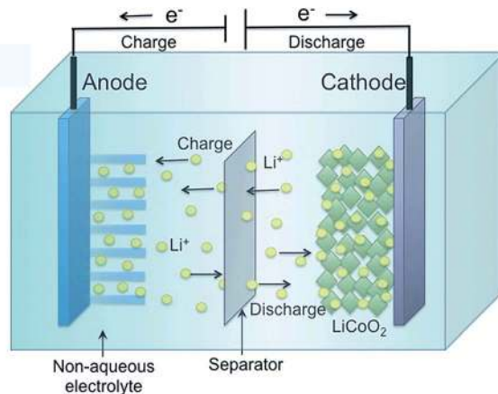
Fig. 1 Schematic diagram of the lithium intercalation-de-intercalation reaction mechanism in a rechargeable lithium-ion battery containing solid electrodes and a liquid electrolyte. Reproduced with permission from ref. 7. Copyright 2015, J. Mater. Chem. A .
