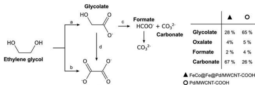
Fig. 17 Proposed reaction pathway for EG electro-oxidation on \text{FeCo@Fe@Pd/MWCNT-COOH} and \text{Pd/MWCNT-COOH} in alkaline medium. Figure adapted from ref. 26 with permission.
