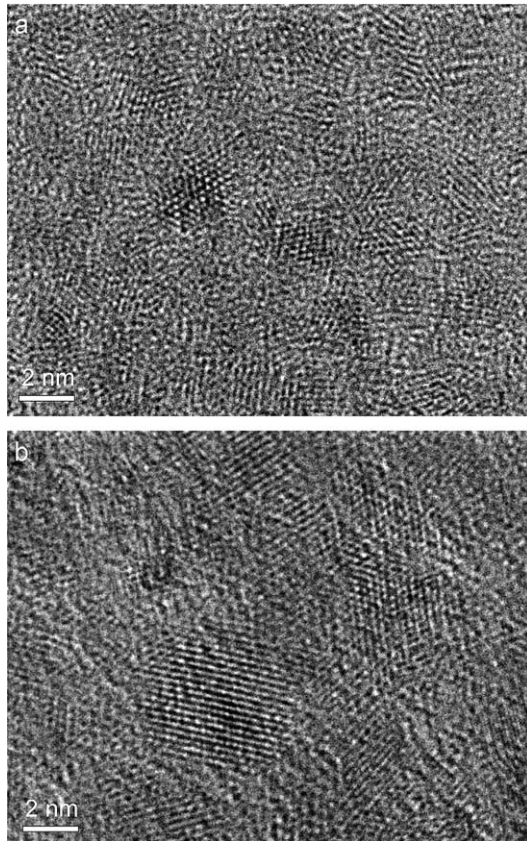
Fig. 4. HRTEM micrographs showing TiC nanocrystallites embedded in a-C:H matrix in nc-TiC/a-C:H nanocomposite: (a) coating HB3 with 17.84 at.% Ti and (b) coating HB5 with 31.75 at.% Ti.
