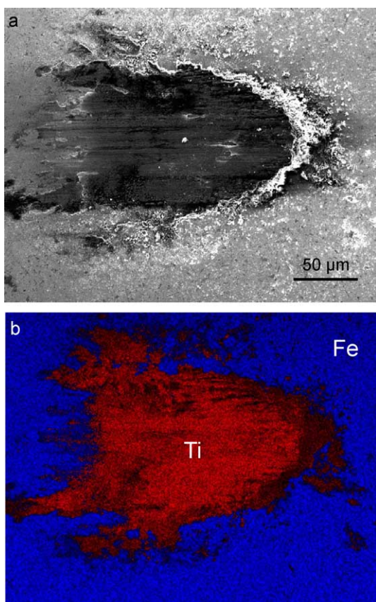
Fig. 7. SEM elements mapping reveals transfer films on the contact area of steel ball from nc-TiC/a-C:H coatings: (a) SEM micrograph of the contact area and (b) Ti and Fe element mapping.
