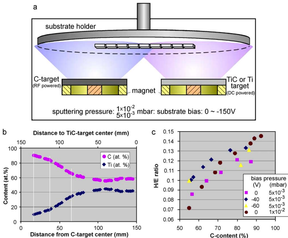
Fig. 1. (a) Sketch of setup for deposition of nc-TiC/a-C coatings; (b) C/Ti content gradient achieved in a batch deposited at -40 V substrate bias and 5 \times 10^{-3} mbar pressure and (c) H/E ratio vs. carbon content under various deposition conditions.
