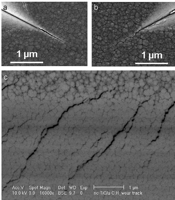
Fig. 5. Radial cracks induced by nanoindentation in the coating HB3 (a) and HB5 (b). (c) Surface fatigue cracks formed in a wear track on the coating HB5.
