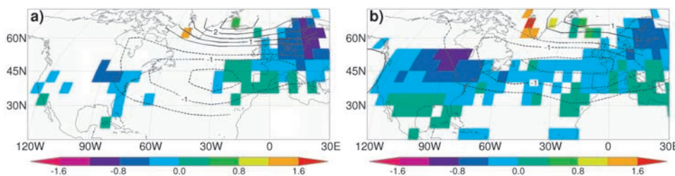
Figure 2. The spatial response of surface pressure (contours in hPa) and temperature (scale in ^{\circ}C ) corresponding to a 1\sigma increase in the ice core PC1 time series. (a) is based on a linear regression of the PC1 time series versus CRU Dec–Mar surface pressure and temperature data for 1874–1970 and 1857–1970 (year of Jan) respectively. (b) as for (a) but only for Dec–Mar 1897–1926 (see text for details). Grid points with more than 10% missing temperature data are left blank.
