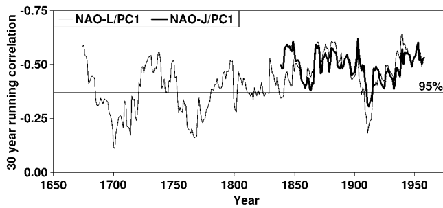
Figure 3. Running 30 year Pearson correlations between the ice core PC1 time series and December to March means of the NAO-L and NAO-J indices. Correlations numerically larger than 0.36 are significant at the 95% level.
