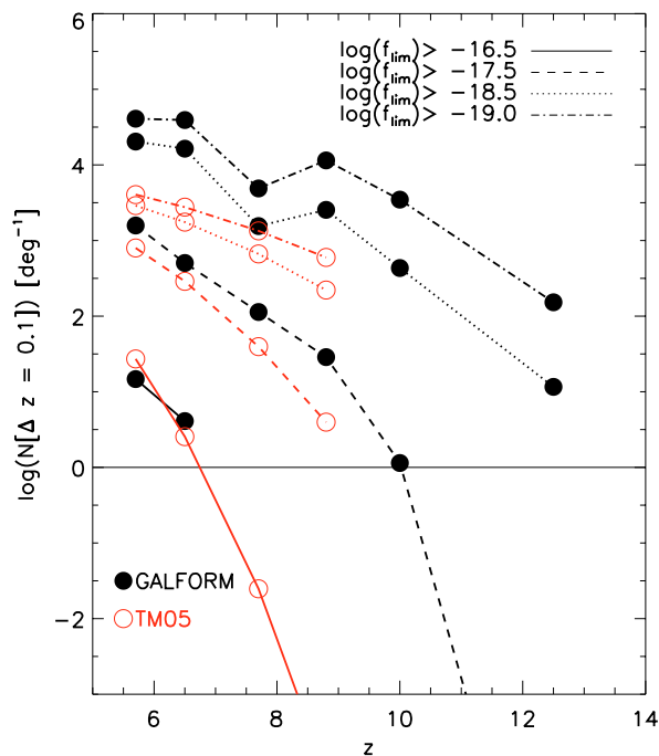
Fig. 4. Summary of predictions. The plot shows the number of \text{Ly}\alpha emitting galaxies expected per square degree per redshift interval \Delta z = 0.1 as a function of redshift and observed flux limit. The predictions of GALFORM are shown in black and of the TM05 model in red. The different line styles are for different flux limits.
