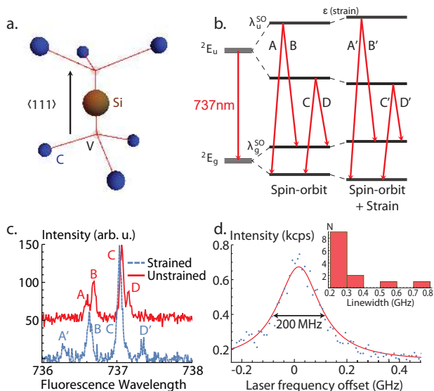
FIG. 1. Properties of the \text{SiV}^- center. a. Atomic structure of the \text{SiV}^- center. The V-Si-V axis lies along the (111) lattice direction. The \text{SiV}^- has D_{3d} symmetry. b. Level structure of the \text{SiV}^- center. The \text{SiV}^- is a single-hole system with double orbital and spin degeneracy. This degeneracy is partially lifted by spin-orbit coupling ( \lambda_g^{SO} = 47 GHz and \lambda_u^{SO} = 260 GHz[11, 15]). Lattice strain increases the splitting between these spin-orbit levels, shifting the transition frequencies. c. Fluorescence spectra of the ZPLs of single \text{SiV}^- centers in high-strain (blue, dashed) and low-strain (red) environments at 9–15 K. Transitions B and C are less sensitive to strain compared with transitions A and D because the ground and excited states shift in the same (opposite) directions for transitions B and C (A and D)[12]. Unstrained spectrum offset and scaled vertically for clarity. d. Linewidth (FWHM) of representative implanted \text{SiV}^- in bulk (unstructured) diamond measured by PLE spectroscopy (blue points: data; red line: Lorentzian fit). Inset: histogram of emitter linewidths in bulk diamond. Almost all emitters have a linewidth within a factor of three of the lifetime limit (94 MHz).
