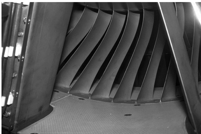
Figure 35.—GE swept and leaned stators tested on CFM-56 engine.
