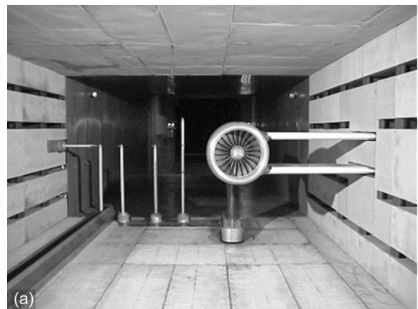
Figure 37.—Alternative Low Noise Fan (ALNF).
