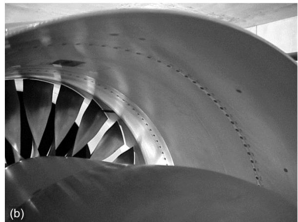
Figure 38.—Source diagnostics test (SDT). (a) External nacelle support struts. (b) Fan with no stators; view looking toward inlet from aft bypass duct.
