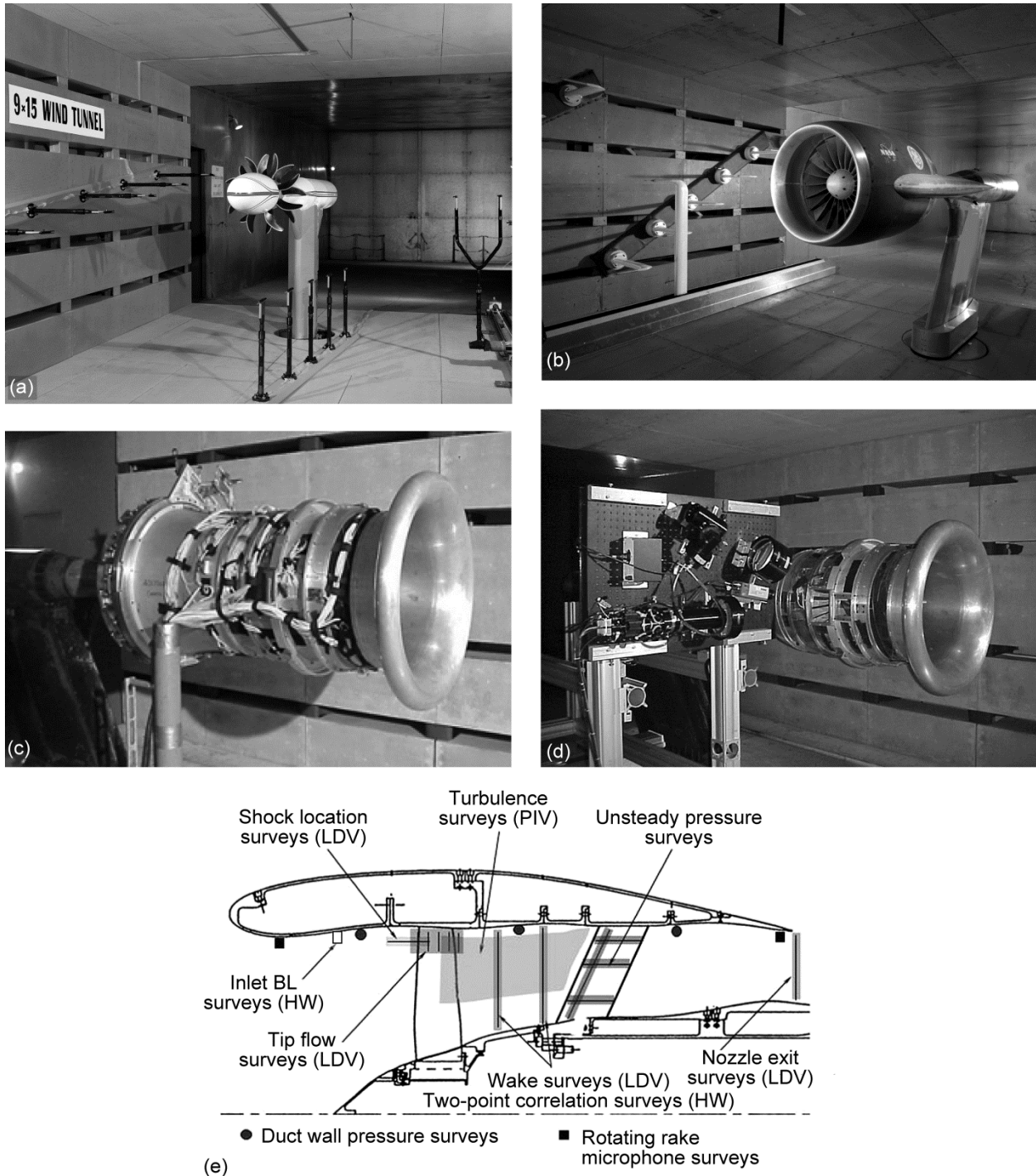
Figure 10.—Model tests in the 9- by 15-Foot Low-Speed Wind Tunnel (9x15 LSWT). (a) Counterrotation propfan, acoustic configuration. (b) Ducted fan, acoustic configuration. (c) Aerodynamic configuration. (d) Laser Doppler velocimetry. (e) Suite of flow and noise measurements.
