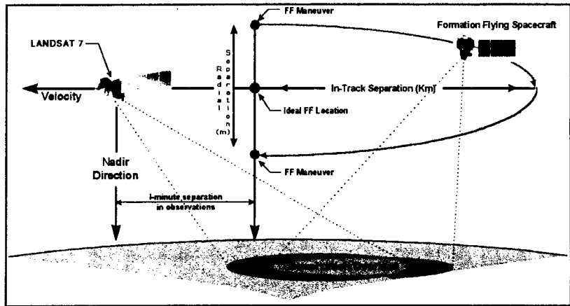
Figure 1. EO-1 Formation Relative Motion
