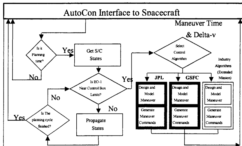
Figure 2. AutoCon Control Flow
