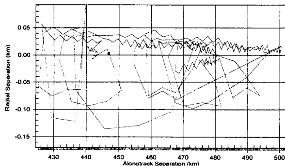
Figure 3. EO-1 Formation Evolution
