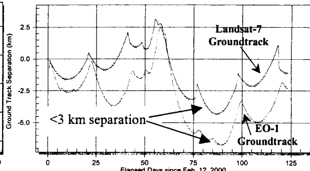
Figure 4. EO-1 and Landsat-7 Relative Groundtrack
