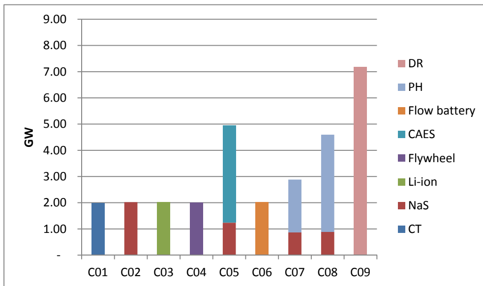
Figure 8.23. Power Requirements for all the Technologies to Meet Balancing Signal for NWPP
