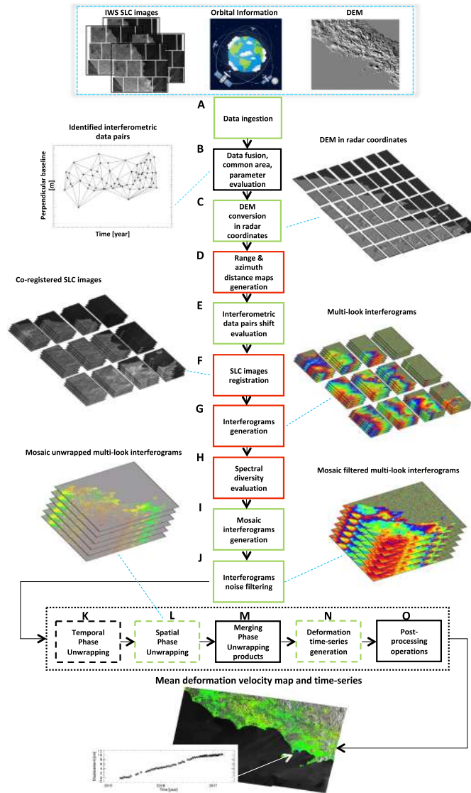
Fig. 1. Block diagram of the S1 P-SBAS processing chain. Green and red blocks represent the processing steps that are executed in parallel by splitting the computation on subsets of input data (subsets of bursts, subsets of SLC images, interferograms or other interferometric products). Dashed line blocks represent processing steps benefiting also from multi-threading programming. Black blocks stand for the processing steps that are sequentially executed.
