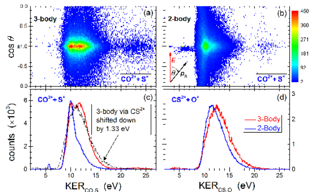
FIG. 4. (Color online) First step of \text{OCS}^{3+} sequential fragmentation. Yield of \text{CO}^{2+} + \text{S}^+ as a function of \text{KER}_{\text{CO,S}} and \cos\theta for (a) three-body and (b) two-body breakup. Yield of (c) \text{CO}^{2+} + \text{S}^+ and (d) \text{CS}^{2+} + \text{O}^+ as a function of KER (scaled by peak height).
