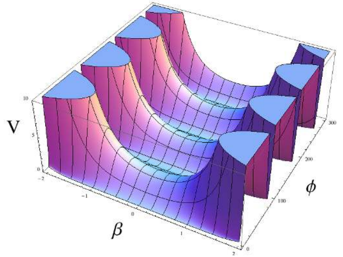
FIG. 1. Potential of the natural inflation model (7) in supergravity at S = 0 and T = \frac{\beta+i\phi}{\sqrt{2}} . During inflation \beta = 0 at its minimum and \phi is the inflaton field with the potential (1). This plot is made for a = 0.1 . All fields are given in Planck units, and the potential is in units \Lambda^4 .
