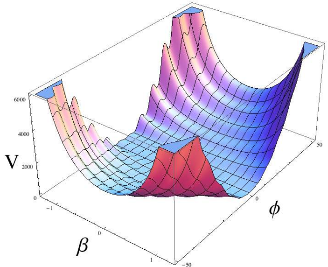
FIG. 4. Potential of the modulated chaotic inflation in supergravity (30) at S = 0 and T = \frac{\beta+i\phi}{\sqrt{2}} , for a = 1 , b = 1.3 . It is similar to the potentials encountered in axion monodromy models [9, 10]. Fields are shown in Planck mass units, the scale of the potential is in units \Lambda^4 .
