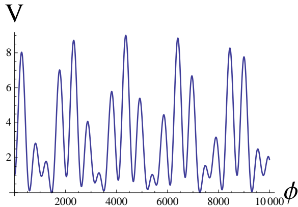
FIG. 2. Irrational axion potential for A = B = 1 , a = 0.01\sqrt{3} , b = 0.005\sqrt{7} . The field is shown in Planck units, from 0 to 10000. This may create an impression that the potential is very steep, but in fact the potential is very flat and allows chaotic inflation. Just as in the string landscape scenario [12–17], inflation may end in any of the infinitely many metastable dS vacua with different values of the cosmological constant [18].
