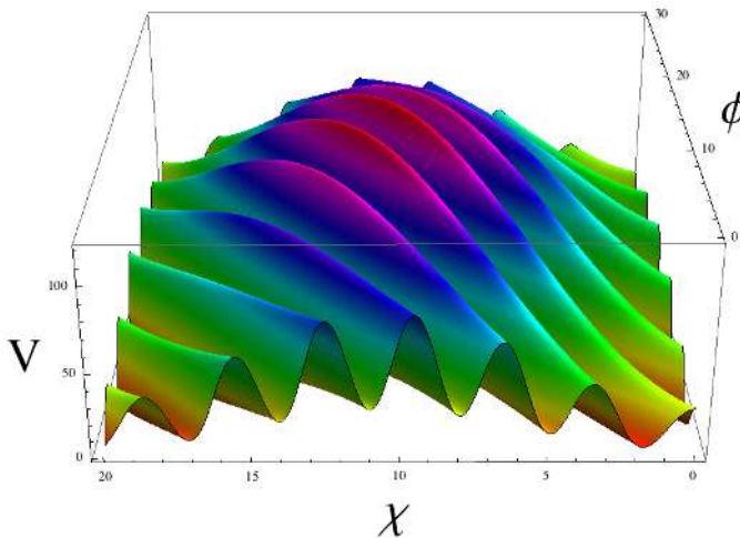
FIG. 3. Inflationary potential for natural inflation in the theory of two scalar fields, T = \frac{\beta+i\phi}{\sqrt{2}} and U = \frac{\gamma+i\chi}{\sqrt{2}} , as a function of the fields \phi and \chi . The potential shown in units of \Lambda^4 , with all other parameters of the superpotential O(1) . Nevertheless, flat inflationary valleys are formed for |a - b| \ll 1 or |c - d| \ll 1 .
