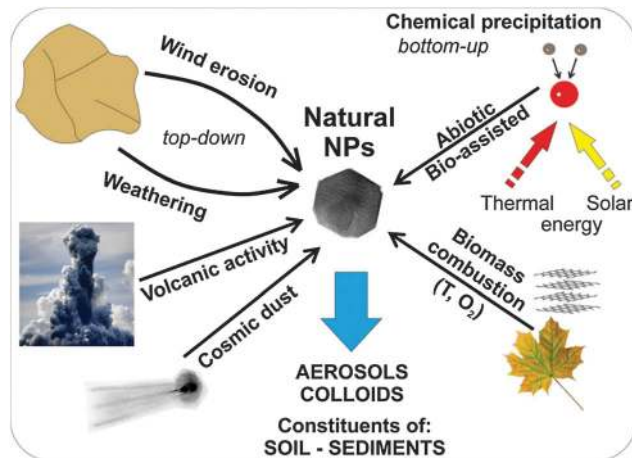
Fig. 3 Natural processes leading to the formation of nanoparticles in the environment. (Natural NPs – natural nanoparticles; T – temperature; O 2 – oxygen).
