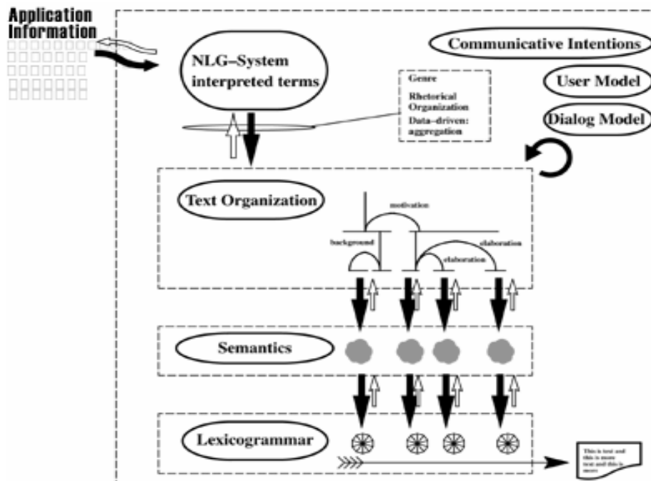
Fig. 1. Abstract Generation System
