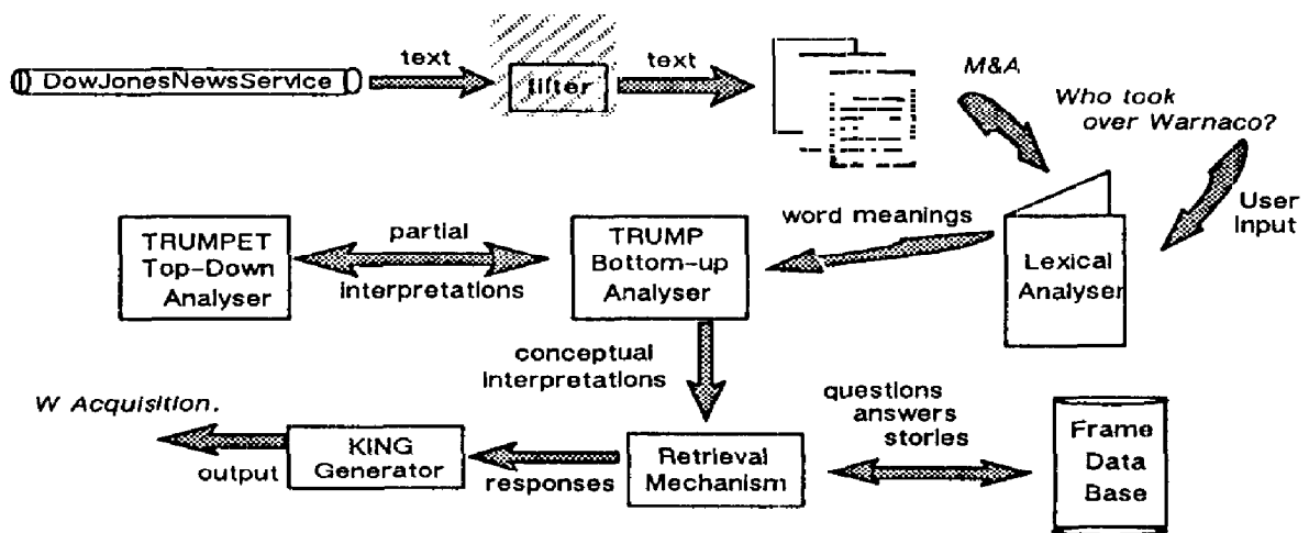
Figure 1: SCISOR System Architecture
