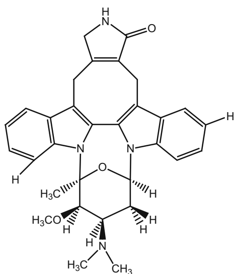
279_4'-N-methylstaurosporine
