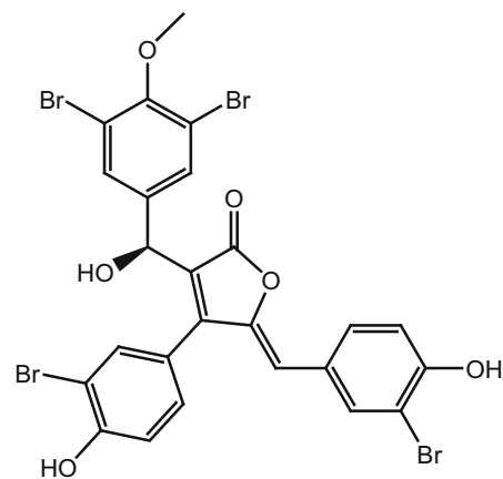
103_cadiolides_F
