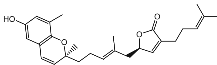
484 _Tuberatolide B
