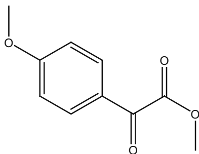
425_methyl 2-(4-methoxyphenyl)-2-oxoacetate
