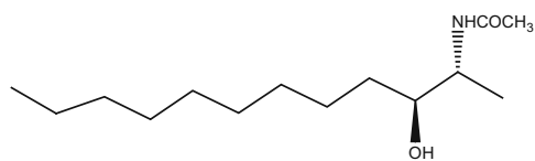
355_clavaminol C
