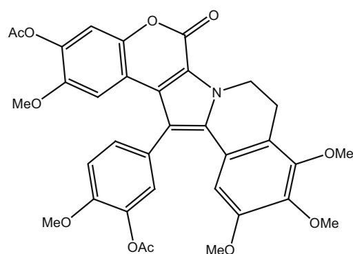
329_lamellarin-T diacetate
