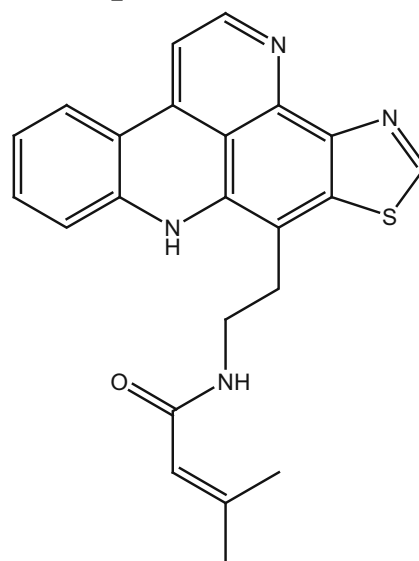
321_dehydrokuanoniamine B
