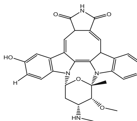
283_3-hydroxy-7-oxostaurosporine
