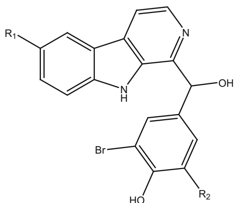
110_Eudistomin Y9; R 1 = Br, R 2 = H
