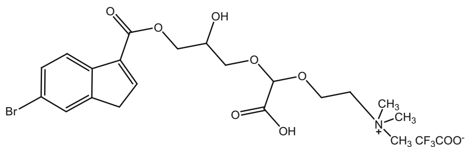
348_durabetaine B
