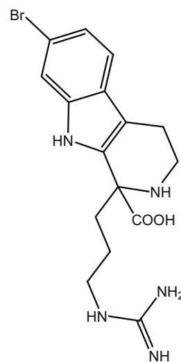
173_1-carboxytryptargine
