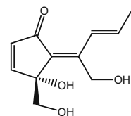
464_cyclopentenones 1
