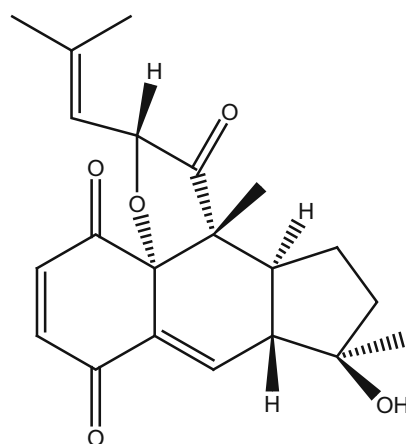
98_3-Epi-rossinone B
