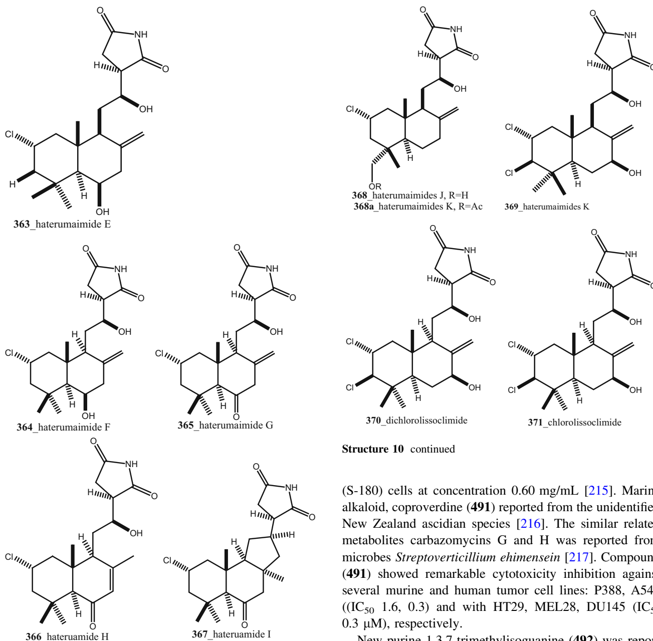
Structure 10 continued
