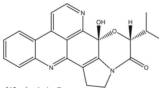
315_sebastianine B
