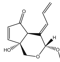
467_cyclopentenones 4
