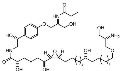
79_Shishididemniol A
