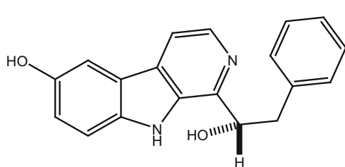
63_Eudistomins W
