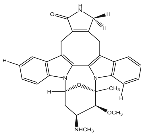
272_11-Hydroxystaurosporine
