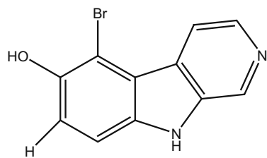
308_eudistomins D
