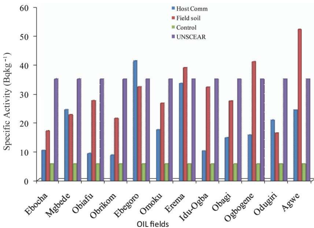
Figure 2 Comparison of 226 Ra Activity in Host Comm. Soil, and Field Soil with UNSCEAR, 2000
