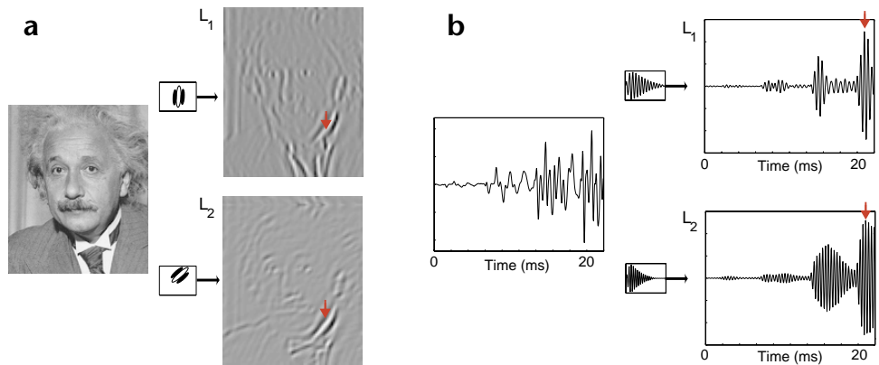
Fig. 1. Linear filter responses to example image and sound stimuli.
