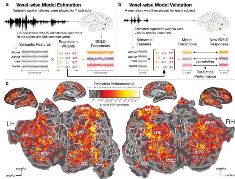
Figure 1. Voxel-wise modeling
