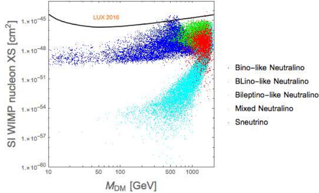
Figure 11. Spin-independent WIMP-nucleon scattering cross section generated in our scan against the upper bounds from 2016 run of the LUX experiment.
