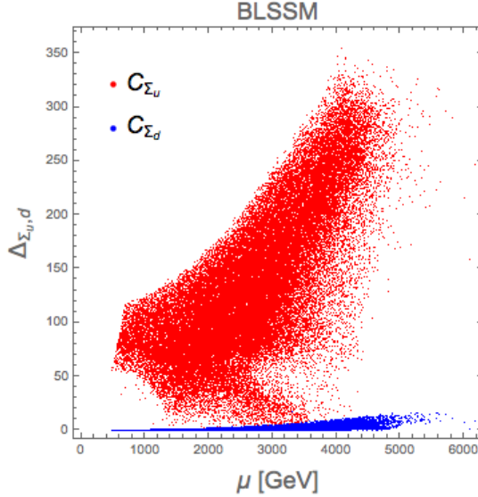
Figure 7. SUSY-FT for for one-loop tadpole corrections C_{\Sigma_u} and C_{\Sigma_d} for given values of \mu . Their contribution is never dominant and so loop corrections do not affect the SUSY-FT.
