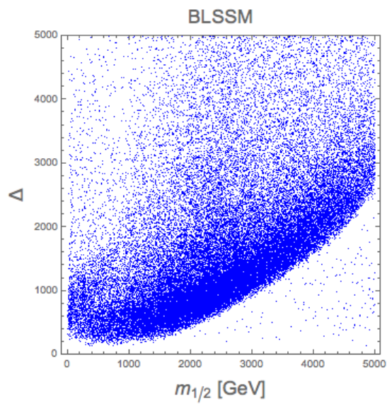
Figure 8. GUT-FT plotted against m_{1/2} . There is a strong, dependence for the GUT-FT with the m_{1/2} parameter, although the wide upward spread indicates other parameters may also be the dominant FT contribution.
