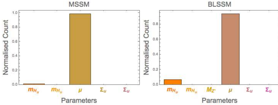
Figure 5. SUSY-FT histogram for the MSSM (left) and BLSSM (right), showing contribution of SUSY parameters.
