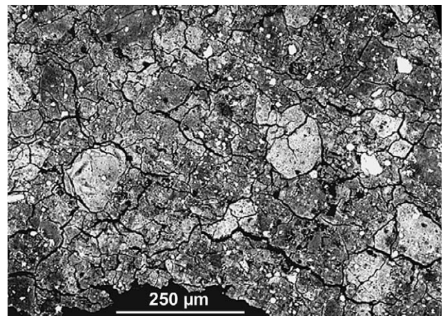
Fig. 8. Part of the severely brecciated CI chondrite Orgueil. Individual fragments are variable in composition as indicated by different gray tones. Image in backscattered electrons; modified after Morlok (2002).
