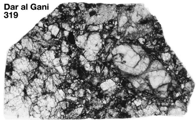
Fig. 13. Overview photograph of the polymict ureilite DaG 319 showing the fragmented character of the sample (1.4 cm in largest dimension).
