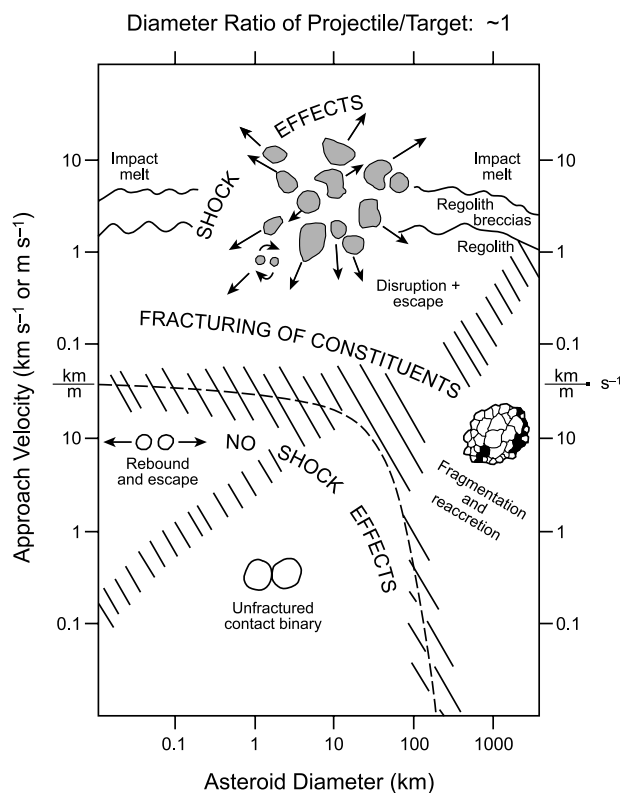
Fig. 1. Regimes of collision-induced effects as a function of the approach velocity (velocity of infinity) and the size of the colliding bodies: Equal-sized bodies are assumed. Minimum velocities for the onset of certain shock effects in meteorites (e.g., formation of impact melts and regolith breccias) are given in wavy lines. The diagram is modified and redrawn from Hartmann (1979) and Stöffler et al. (1988).
