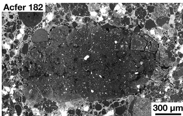
Fig. 11. Dark inclusion in the CH chondrite Acfer 182. The fine-grained inclusion contains some large pyrrhotite grains (white) and abundant pores (dark spots) and fractures. Photomicrograph in backscattered electrons; cf. Bischoff et al. (1993b).
