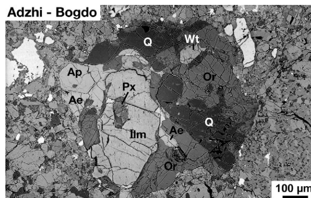
Fig. 5. Alkali-granitoid clast from Adzhi-Bogdo (LL3–6) ordinary chondrite regolith breccia consisting of apatite (Ap), aenigmatite (Ae), ilmenite (Ilm), whitlockite (Wt), quartz (Q), and K-feldspar (Or). Within quartz tiny grains of zircon are enclosed (white). Photomicrograph in backscattered electrons (cf. Bischoff et al., 1993c; Bischoff, 1993).
