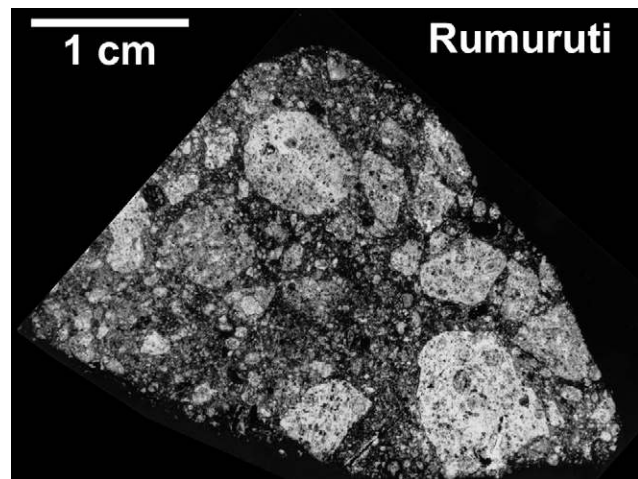
Fig. 6. Overview of the R chondrite regolith breccia Rumuruti. The photographed hand specimen consists of light- and dark-colored fragments embedded in a clastic matrix. The abundance of large clasts is roughly 50%. See Schulze et al. (1994) for details.
