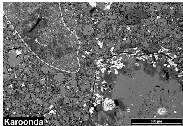
Fig. 10. Brecciated nature of the Karoonda CK chondrite. A fine-grained (upper left) and coarse-grained fragment (lower right) are embedded in a fine-grained clastic matrix. Image in backscattered electrons.
