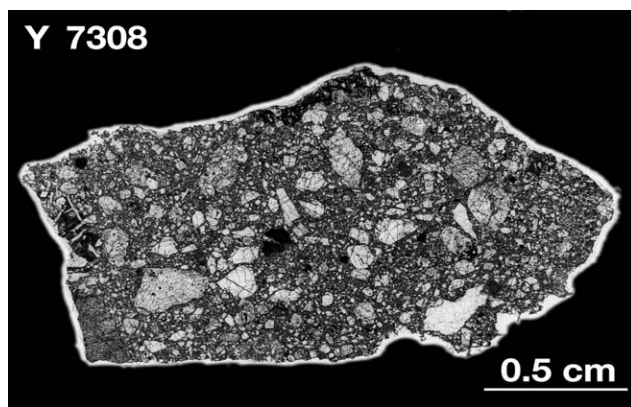
Fig. 14. Overview photograph of the Y-7308 howardite. Different types of fragments are embedded within a fine-grained clastic matrix. Image in transmitted light. See Metzler (1985) for details.
