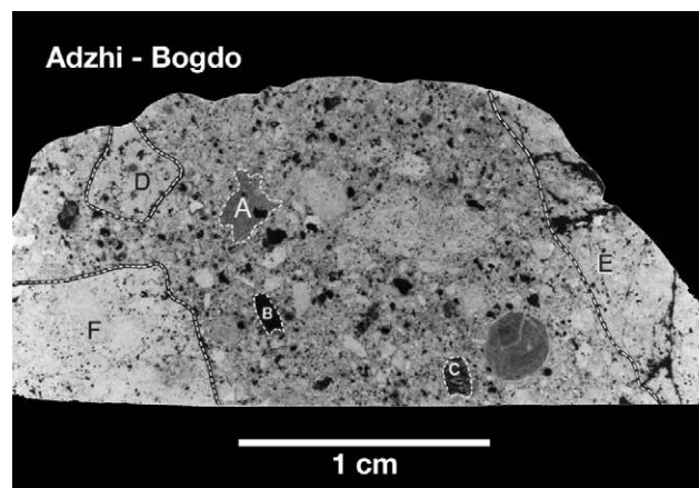
Fig. 2. Transmitted light photomicrograph of a thin section from the Adzhi-Bogdo (LL3-6) chondrite regolith breccia showing various types of fragments: highly recrystallized clasts (D, E, and F) sometimes with internal shock veins (E), melt-rock clast (A), fragmental breccia clast (B), and a shock-darkened fragment (C). After Bischoff et al. (1993c).
