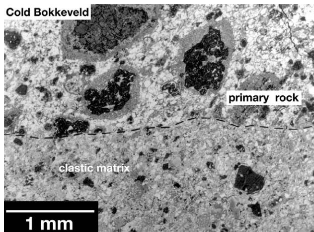
Fig. 9. Typical appearance of a CM breccia as indicated by the boundary between a fragment of primary accretionary rock and the clastic matrix. In the upper part all the coarse-grained components are surrounded by accretionary dust mantles, whereas in the clastic matrix angular fragments occur and all coarse-grained components have lost their dust mantles due to impact-induced fragmentation. Image in backscattered electrons after Metzler et al. (1992).
