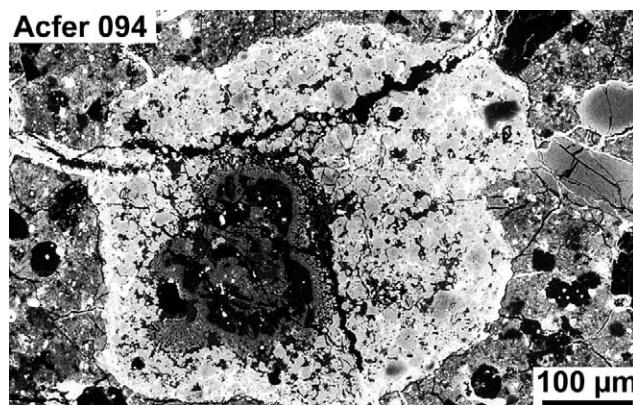
Fig. 12. CAI-bearing lithic fragment in the unique carbonaceous chondrite Acfer 094. This clast contains a Ca,Al-rich inclusion (dark gray; center, lower-left) surrounded by olivine-rich components. Image in backscattered electrons.
