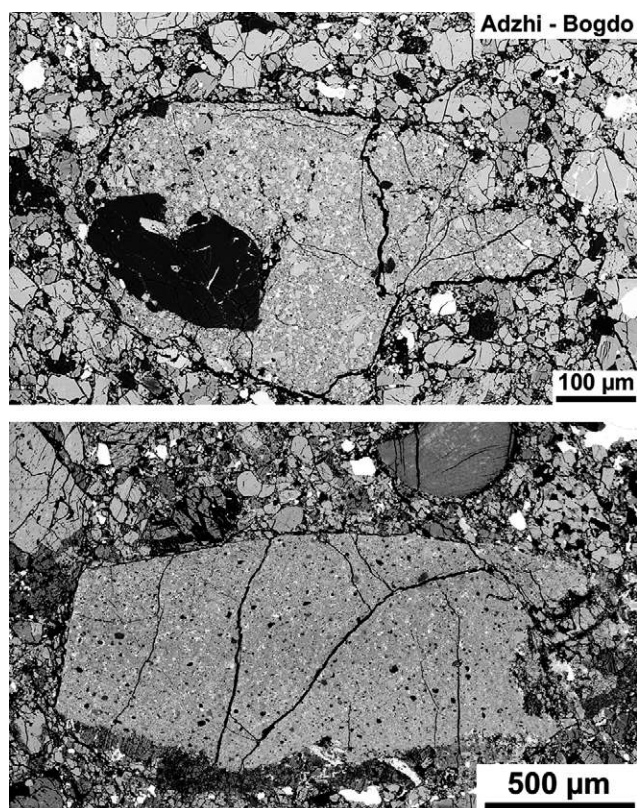
Fig. 4. Backscattered electron image of two fine-grained, optically dark fragments in the Adzhi-Bogdo (LL3–6) ordinary chondrite regolith breccia. Both fragments can be described as individual breccias that occur within the Adzhi-Bogdo host breccia (breccia in a breccia). The large black grain in the upper image is a plagioclase grain ( An_{20} ).
