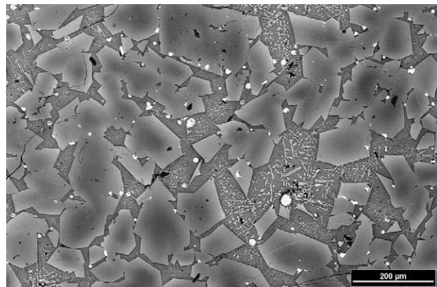
Fig. 7. Typical texture of an impact melt clast within the R chondrite DaG 013. Euhedral to subhedral, zoned olivine grains are embedded in a mesostasis containing tiny, skeletal crystals of pyroxene. Light grains are either chromite or Fe-sulfide. Image in backscattered electrons.
