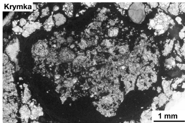
Fig. 3. Fragment of an unusual chondritic fragment in the unequilibrated ordinary chondrite Krymka (LL3). The clast consists chemically of almost equilibrated Mg-rich olivine (Fa: 8.1 \pm 1.6 ) and somewhat more variable pyroxene (Fs: 6.4 \pm 3.3 mol%). Due to the occurrence of abundant opaque grains the fragment has a black appearance at the edge (especially in the lower part). Photomicrograph in transmitted polarized light.
