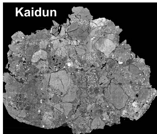
Fig. 15. Kaidun belongs to the most heavily fragmented chondrites showing the huge number of diverse lithologies. Backscattered electron image, 4 cm across, provided by M. Zolensky; see Zolensky and Ivanov (2003) for details.
