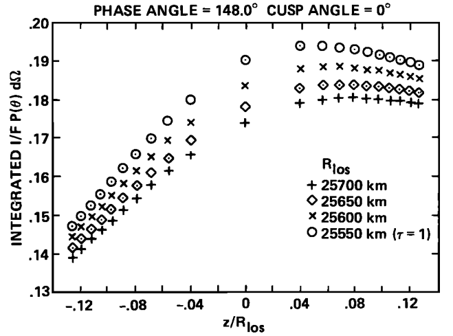
Fig. A2. Magnitude of the source term for planet-reflected light (ordinate) that is scattered in the optically thin part of the atmosphere as a function of distance z from the tangent point for the line of sight (abscissa). In this figure, distance z is normalized by the distance of the tangent point from the planet's center, R_{\text{los}} . Results are shown for four choices of R_{\text{los}} . The optical depth of the atmosphere (for normal incidence) is unity at R_{\text{los}} equal to 25,550 km.
