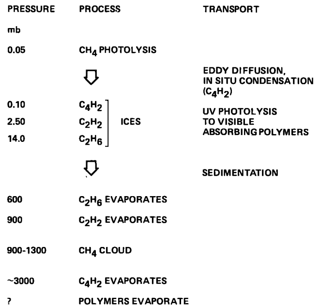
Fig. 9. Schematic diagram of the stratospheric aerosol cycle.
