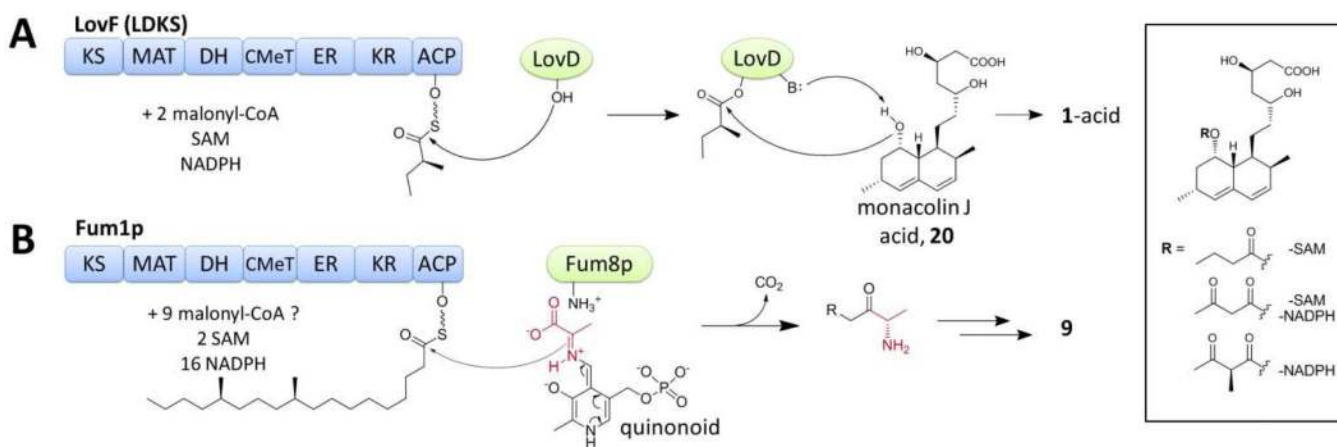
Figure 3. Off-loading of reduced linear polyketide product synthesized by HR-PKSs. (A) LovD acyltransferase-mediated offloading in biosynthesis of 1 . Lovastatin derivatives obtained by in vitro feeding of diketide SNAC substrates were shown in the box. (B) FUM8p-mediated offloading in biosynthesis of 9 .
