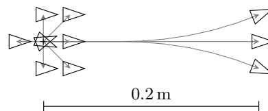
Fig. 4. Omnidirectional motion primitives for the PR2.
