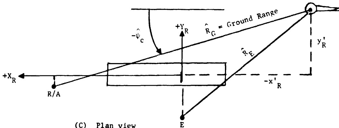
Figure 7. Geometry of MLS Navigation
