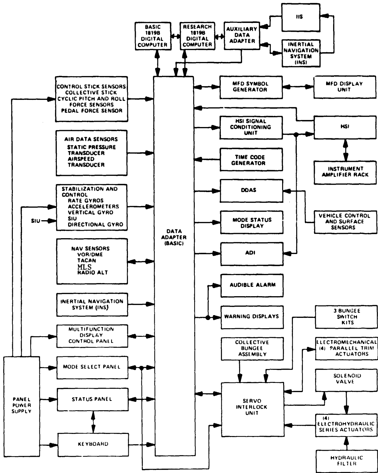
Figure 1. UH-1H V/STOLAND System Block Diagram
