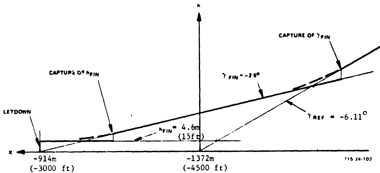
Figure 4. Final Vertical Guidance Geometry
