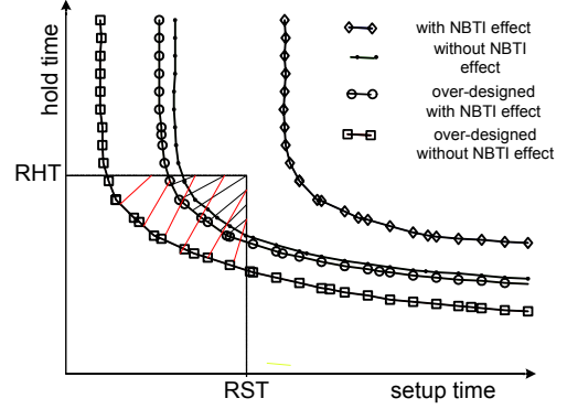
Figure 7. Flip-flop design.
