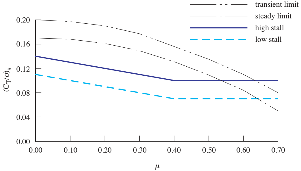
Figure 12-7. Stall function.
