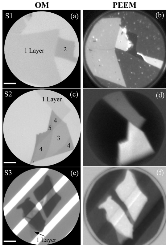
FIG. 1. OM images [(a), (c), and (e)] and PEEM ones [(b), (d), and (f)] of some selected samples (S1, S2, and S3). Scale bars are: 5 \mu\text{m} in (a) and (e); 10 \mu\text{m} in (c).
