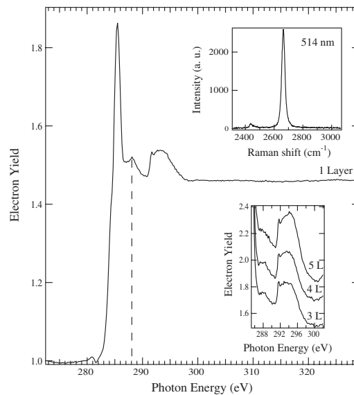
FIG. 4. C K -edge photoabsorption spectra of graphene taken from sample S2. Upper inset: the Raman spectrum of graphene at 514 nm showing the single component of the 2D peak. Lower inset: close-up of photoabsorption spectra extracted from sample S2.
