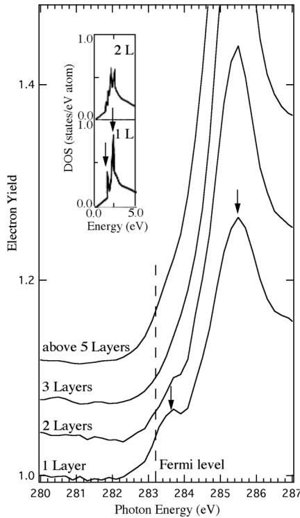
FIG. 3. Expanded C K -edge photoabsorption spectra extracted from Fig. 2. The inset shows DOS calculations of single- and double-layer graphene [8], in the energy region (0.0–5.0) eV above E_F . The Fermi level, as extracted from Ref. [8], is also reported in the graph. Arrows show the double structure of the \pi^* resonance in graphene. The separation between the two features in the theoretical DOS of single-layer graphene is about 0.8 eV, while the experimental separation is between 1.2 and 1.8 eV for our samples.
