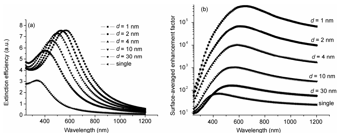
Figure 2 Incident wavelength dependent spectra of a single Pd nanosphere and Pd nanosphere dimers with D = 100 nm and various d . (a) Extinction efficiency; (b) surface-averaged SERS enhancement factor.
