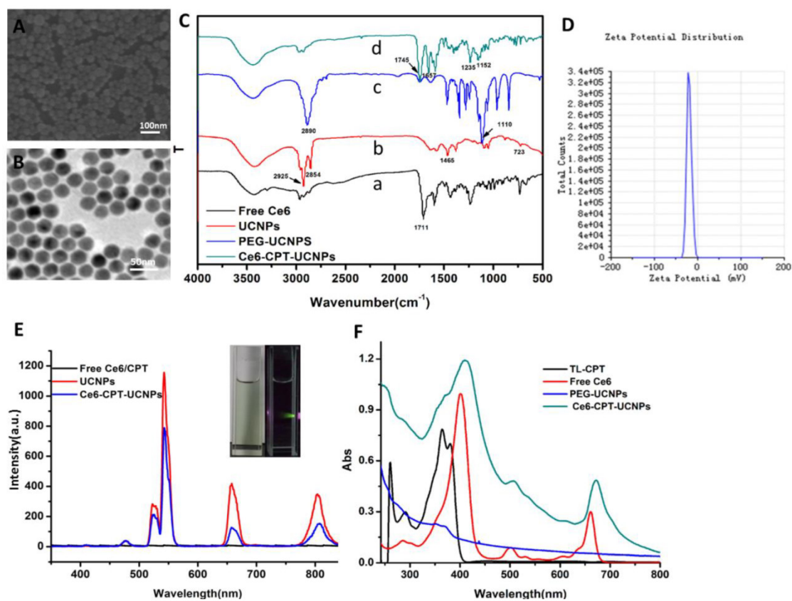
Figure 2. Characterization of Ce6-CPT-UCNPs.(A)SEM image of UCNPs.(B) TEM image of UCNPs. (C) FTIR spectra of (a) Free Ce6, (b) UCNPs, (c) PEG-UCNPs, and (d)Ce6-CPT-UCNPs.(D)Zeta potential of Ce6-CPT-UCNPs, the zeta potential was about -19.8mV. (E) Upconversion luminescence spectra of free Ce6/CPT in DMF,UCNPs (2mg/mL) and Ce6-CPT-UCNPs (2mg/mL) in water, excitation:980 nm.(F) Normalized UV/vis absorption spectra of TL-CPT (thiokeetal linker conjugated with camptothecin), free Ce6, PEG-UCNPs, and Ce6-CPT-UCNPs,TL-CPT detected in DMSO solution, others dissolved in methanol.
