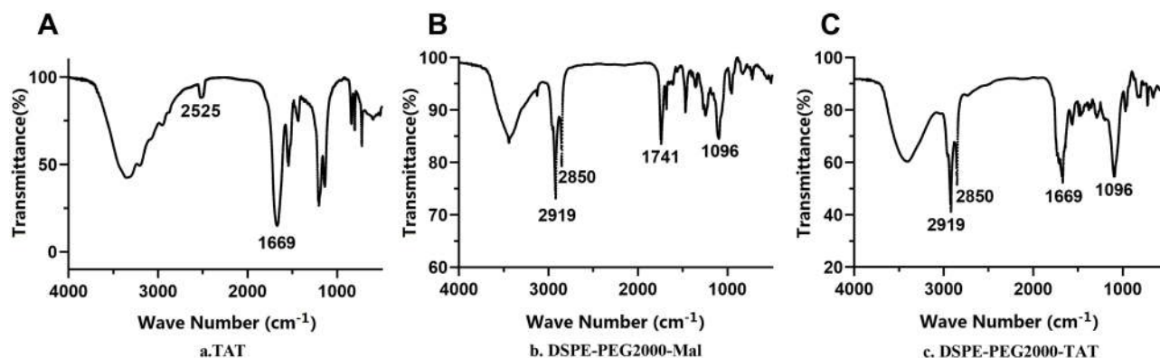
Figure 1 Infrared spectra of (A)TAT and (B)DSPE-PEG2000-Mal before TAT reaction, (C)DSPE-PEG2000-TAT after TAT reaction.
