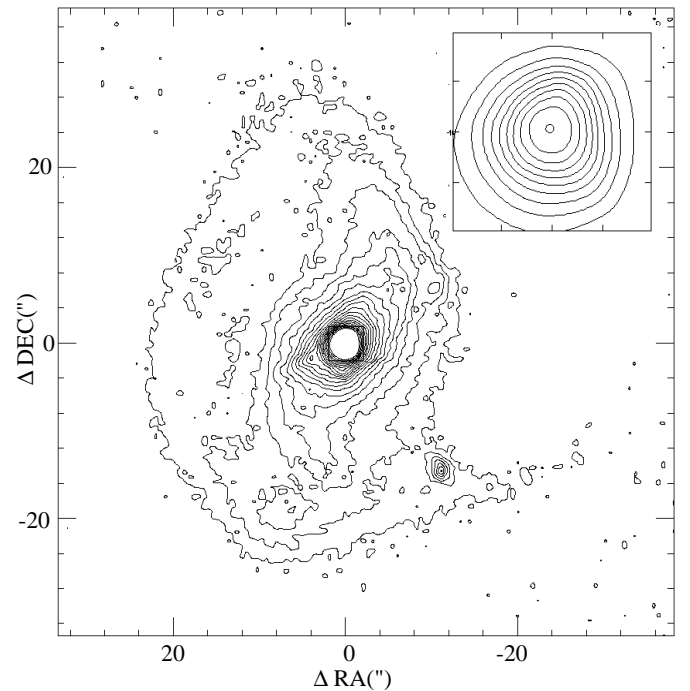
Fig. 9. The K -band image of NGC 7714 with logarithmic intervals. The inset shows the central 4'' \times 4'' region. There is a foreground star toward SW of the nucleus
