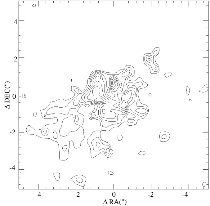
Fig. 11. The \text{H}_2 emission of NGC 7714. The lowest contour is at 31% level of the maximum and corresponds to 3\sigma . The other contours are at 1\sigma intervals. The maximum surface brightness is 5.9 \cdot 10^{-16} \text{ erg s}^{-1} \text{ cm}^{-2} \text{ arcsec}^{-2}
