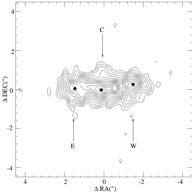
Fig. 2. The \text{Br}\gamma emission of NGC 520 PN. The lowest contour is at 19% level of the maximum and corresponds to 3\sigma . The other contours are at 1\sigma intervals. The maximum surface brightness is 2.4 \cdot 10^{-15} \text{ erg s}^{-1} \text{ cm}^{-2} \text{ arcsec}^{-2} . The black dots correspond to the three \text{Br}\gamma emission regions studied in this work
