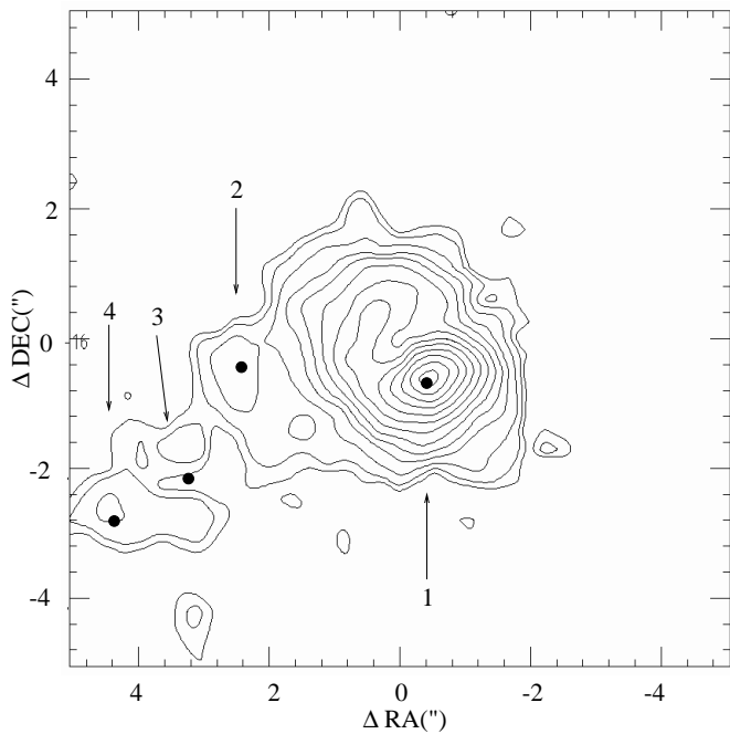
Fig. 10. The \text{Br}\gamma emission of NGC 7714. The lowest contour is at 4.1% level of the maximum and corresponds to 3\sigma . The other contours are at 5.4, 8.2, 12, 16, 22, 29, 46, 57, 69, 83 and 98% of the maximum. The maximum surface brightness is 7.0 \cdot 10^{-15} \text{ erg s}^{-1} \text{ cm}^{-2} \text{ arcsec}^{-2} . The black dots correspond to the four \text{Br}\gamma emission regions studied in this work
