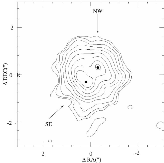
Fig. 6. The \text{Br}\gamma emission of NGC 1614. The lowest contour is at 7.1% level of the maximum and corresponds to 3\sigma . The other contours are at 9.5, 14, 21, 31, 43, 57, 74 and 86% of the maximum. The maximum surface brightness is 7.5 \cdot 10^{-15} \text{ erg s}^{-1} \text{ cm}^{-2} \text{ arcsec}^{-2} . The black dots correspond to the two \text{Br}\gamma emission regions studied in this work
