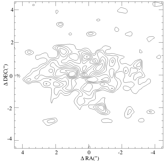
Fig. 3. The \text{H}_2 emission of NGC 520 PN. The lowest contour is at 28% level of the maximum and corresponds to 3\sigma . The other contours are at 1\sigma intervals. The maximum surface brightness is 0.93 \cdot 10^{-15} \text{ erg s}^{-1} \text{ cm}^{-2} \text{ arcsec}^{-2}
