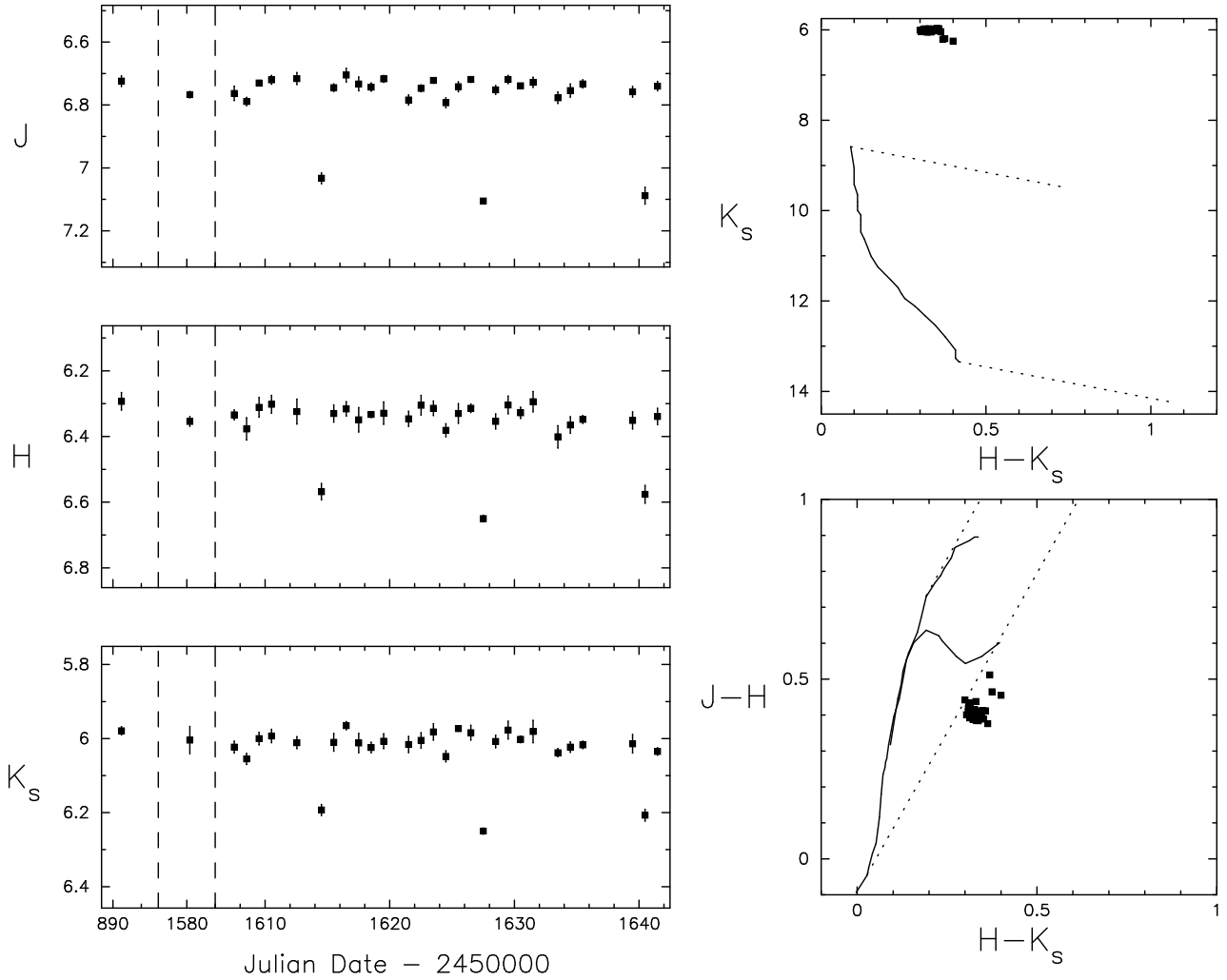
Fig. 6.— Photometric data for star 8783 (also known as BM Ori), classified as an eclipsing system based on the simultaneous drops in the J , H , and K_s magnitudes on 3 discrete days. This eclipsing system was identified previously from optical observations (see, e.g., Antokhina, Ismailov, & Cherepashchuk 1989 and references therein).
