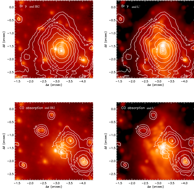
Fig. 8. 2 \mu\text{m} -band image (left; IB 2.15 \mu\text{m} ) and L' -band image (right; 3.8 \mu\text{m} ) with the Br \gamma emission (top) and CO absorption (bottom) line maps in contours overlotted.
