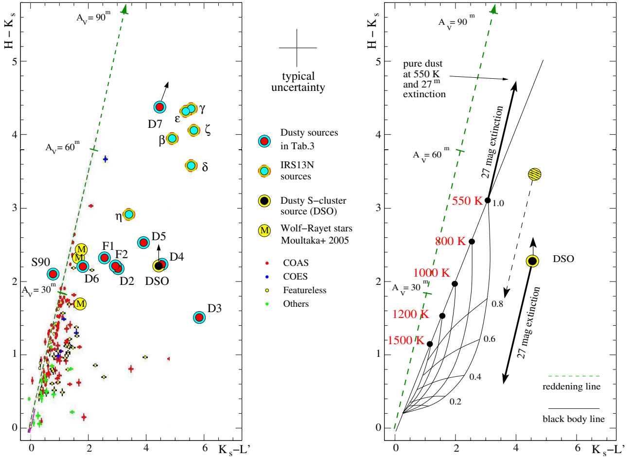
Fig. 16. Left: colors of dusty objects in the central parsec of the Milky Way compared to the colors of young stellar objects as given by Hoffmeister et al. (2006). The labels COAS and COES indicate that the sources show CO absorption or emission in their spectra. Right: colors of dusty objects in the central parsec of the Milky Way compared to colors of pure dust (temperatures given in red numbers) and mixtures of a stellar and a dust contribution (fractional numbers given in black; see also Glass & Moorwood 1985). Here we demonstrate that a mixture of dust and stellar contribution is possible. Because the H - K_s color of DSO is an upper limit, its NIR emission can be explained as pure dust at 550 K reddened by \sim 27 mag, or as a star embedded in warm dust, e.g., if its color were detected to be H - K_s \sim 3.5 mag (dashed circle), after dereddening by 27 mag, its emission would be consistent with 20% stellar and 80% dust contributions.
