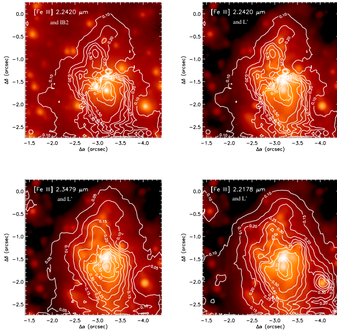
Fig. 9. 2 \mu\text{m} -band image (left; IB 2.15 micron) and L' -band image (right; 3.8 \mu\text{m} ) with [FeIII]-emission line maps in contours overlotted.
