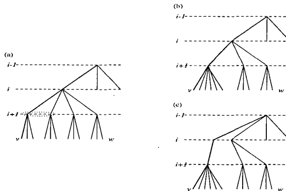
Figure 1: The effect on the structural forest of a replace on level i : Starting from Figure (a), two level i + 1 components are to be merged into the new level i + 1 component T_v containing v . If we find a replacement edge, we go to (b); otherwise we go to (c) and recurse on level i - 1 .
