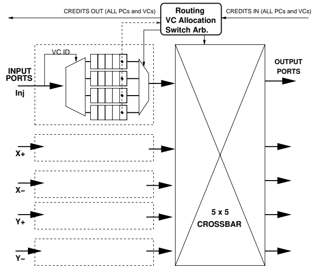
Figure 6: Base Router Model
