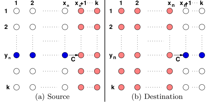
Figure 2: Components of channel load for O1TURN
