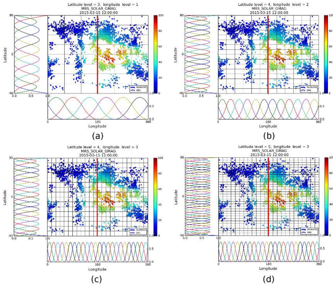
Figure 1. Global VTEC representation in a solar geomagnetic coordinate system using different resolution levels; (a) J_1 = 3 , J_2 = 1 ; (b) J_1 = 4 , J_2 = 2 ; (c) J_1 = 4 , J_2 = 3 ; (d) J_1 = 5 , J_2 = 3 . The circles and triangles represent the data locations for GLONASS and GPS, respectively, and the colors indicate the corresponding VTEC magnitudes related to the ionospheric pierce points (IPP) obtained from a reference map. In all the four panels at the bottom and on the left side the K_{J_2} trigonometric B-spline functions T_{J_2, k_2}^2(\lambda) with k_2 = 0, 1, \dots, K_{J_2} - 1 and the K_{J_1} polynomial B-spline functions N_{J_1, k_1}^2(\varphi) with k_1 = 0, 1, \dots, K_{J_1} - 1 are visualized. The straight black lines on the maps show the corresponding knot point locations. The red line shows the prime meridian at Greenwich.
