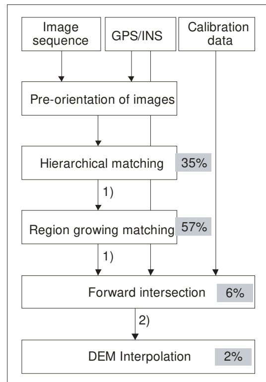
Figure 4 Automatic processing data flow for generation of DSM including calculation time in % and points filtering by 1) cross check by additional matching and by 2) outlier detection during the forward intersection.
