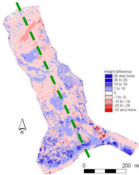
Figure 8 Difference of DSM between the years 2006 and 2007.
