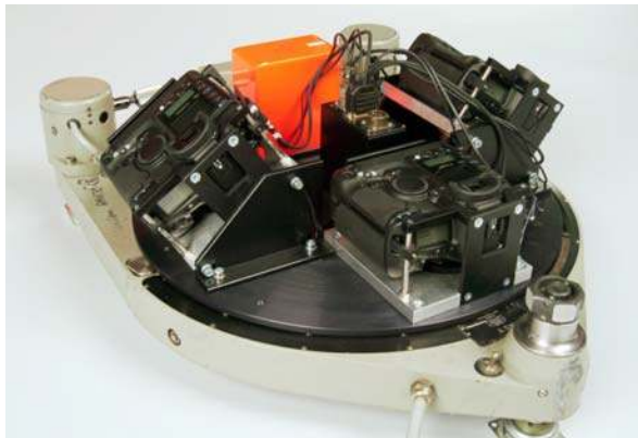
Figure 2 DLR 3K-camera system consisting of three Canon EOS 1Ds Mark II, integrated in a ZEISS aerial camera mount
