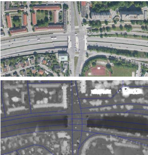
Figure 12 DSM of bridge with road data base segments (bottom) and Orthophoto (top)
