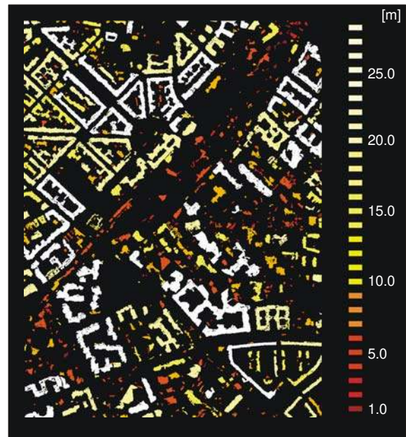
Figure 10 Automatic determination of building heights from 3K DSM
