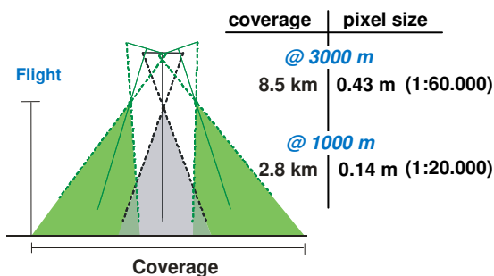
Figure 3 Illustration of the image acquisition geometry. The tilt angle of the sideward looking cameras is approx. 35^\circ .
