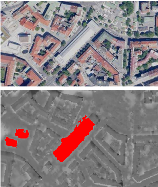
Figure 11 Difference between the 3K DSM from 17 th June 2007 and the LIDAR DEM (bottom) and the corresponding orthophoto (top).
