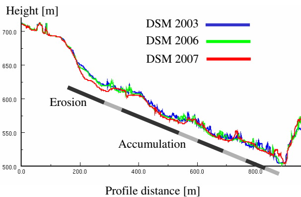
Figure 9 Profile through DSMs of the years 2003, 2006, and 2007.
