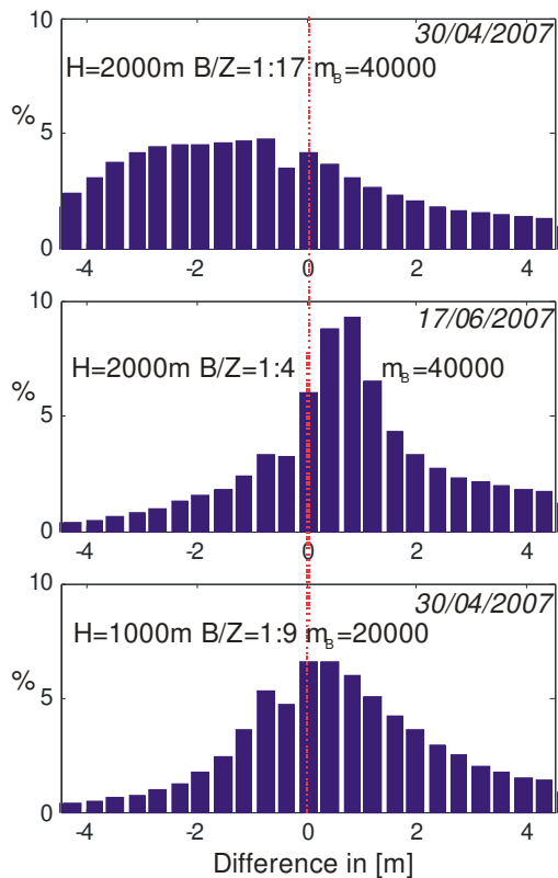
Figure 6 Histogram of DSM difference image (3K DSM minus Reference DEM) for three different data takes over urban area
