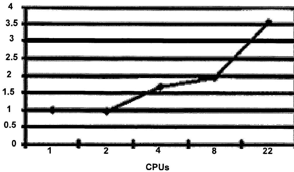
Speedup diagram of the Grid-enabled traffic simulation
