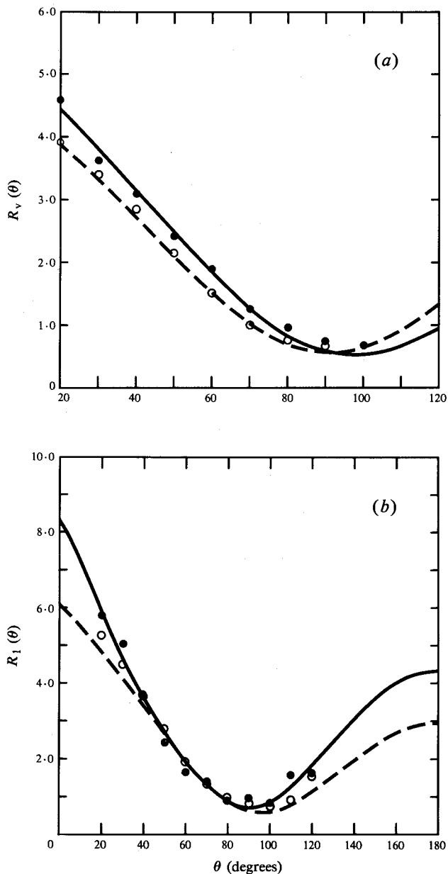
Fig. 10. Ratios of the pure vibrational cross section for \nu_0 = 0 \rightarrow \nu (equation 12) to the ro-vibrational cross sections \sigma_{rv(10,3\nu)}(\theta) : (a) Comparison of theoretical ratios (curves) to data of Wong and Schulz (1974) (symbols) for \nu = 1 (solid curves and solid circles) and \nu = 2 (dashed curve and open circles) at 4.5 eV at T = 298 K; (b) comparison with data of Linder and Schmidt (1971) (symbols) for \nu = 1 at 1.5 eV (solid curve and solid circles) and 2.5 eV (dashed curve and open circles) at T = 340 K.
