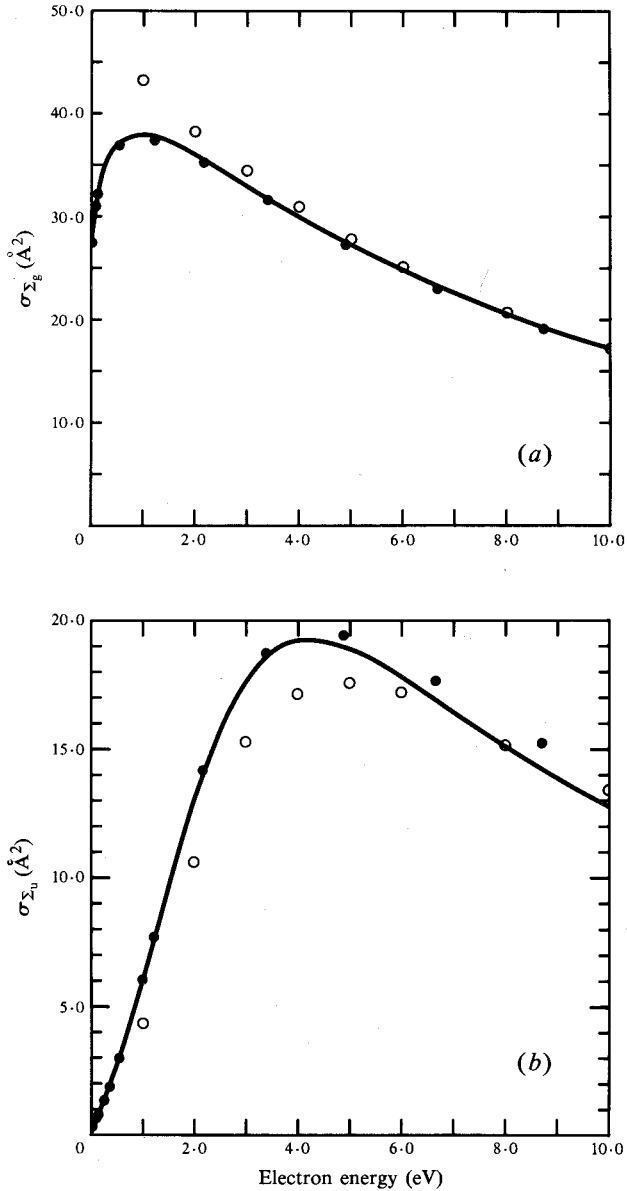
Fig. 16. Assessment of the BTAD polarisation potential in the fixed-nuclei approximation: theoretical partial cross sections for e-H 2 scattering at a fixed internuclear separation R = R_c = 1.402a_0 in the (a) \Sigma_g and (b) \Sigma_u symmetries. Solid curves are results of the present study (see Section 5). The solid circles are cross sections from the optical-potential calculations of Schneider and Collins (1983), and the open circles are from calculations of Gibson et al. (1984) using the Schwinger multichannel method.
