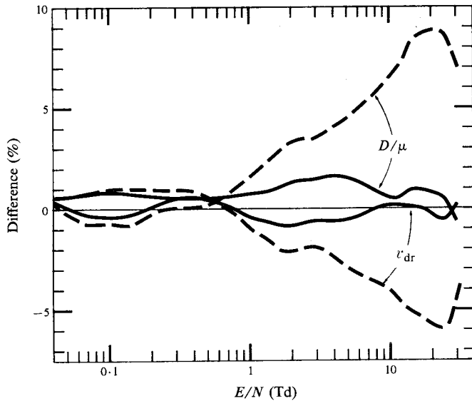
Fig. 18. Differences between the measured values of v_{\text{dr}} and D_{\Gamma}/\mu in H 2 and those calculated using the theoretical cross sections (dashed curves). The corresponding differences when the swarm-derived cross sections are used (full curves) are shown for comparison.
