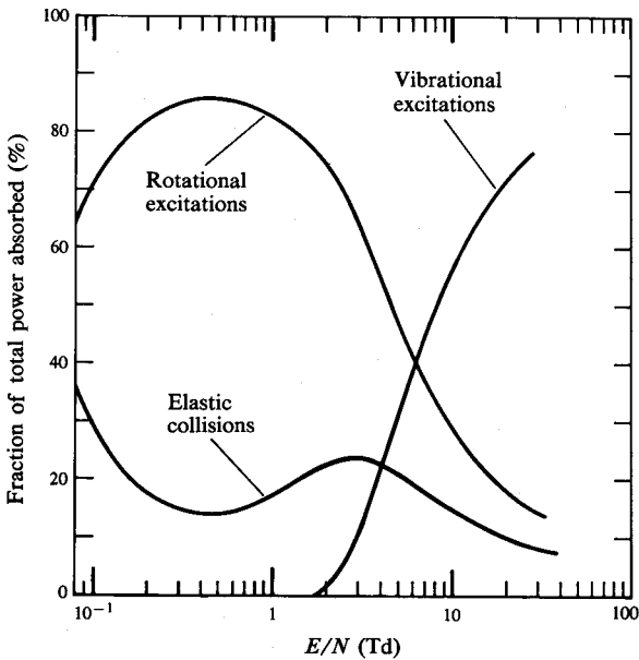
Fig. 3. Fractions of the total power absorbed in elastic collisions and in rotational and vibrational excitation in para-hydrogen at 77 K plotted as functions of E/N . [From Crompton et al. (1969).]
