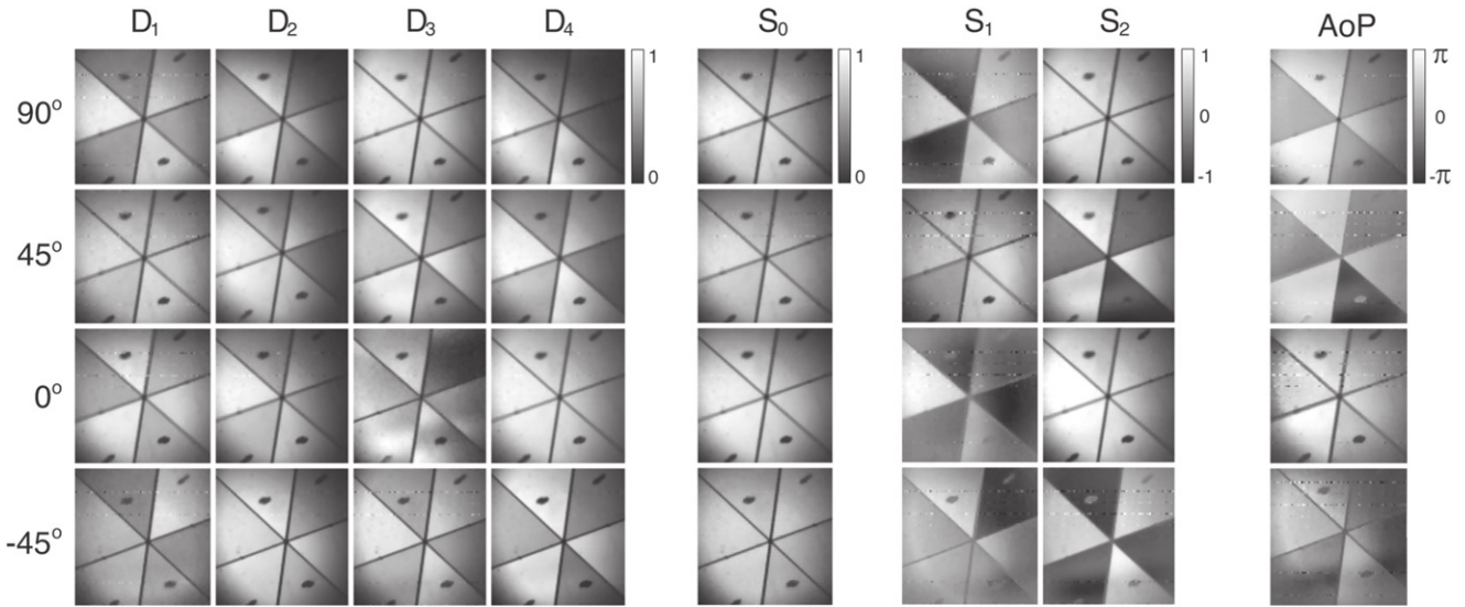
Figure 3. Reconstructed images of a ‘corner cube’ obtained by the polarization sensitive single pixel camera prototype for various incident linear polarization illumination. D1-D4 columns represent the reconstruction from each individual detectors. S_0, S_1 and S_2 columns represent the first three Stokes parameter images obtained through combinations of the signals as described in the main text. The angle of polarization column, AoP, shows the effect of a multi-faceted surface where each mirror ‘segment’ was at a different angle than its neighboring segment, with respect to the linear polarization illumination angle.
