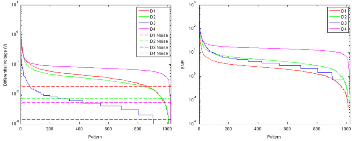
Figure 2. The left figure shows measured signals and associated standard deviation for each detector D1-D4 , plotted in descending order. The right figure shows the associated signal to noise ratio calculated for every pattern. This analysis was performed on a smaller data set containing 1024 patterns. The mean SNR for each detector in a ‘typical’ run is D1 = 2.88 , D2 = 5.89 , D3 = 5.93 and D4 = 15.89 .
